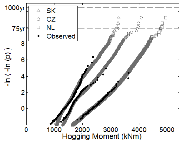
Figure 7. Observed vs. simulated maximum daily load effects for the three European WIM sites. All simulations represent 300 years of traffic (SK = Slovakia, CZ = Czech Republic, NL = Netherlands, AZ = Arizona, IL = Illinois, IN = Indiana). (a) LE1 on a 30-m bridge. (b) LE2 on a 40-m bridge. (c) LE3 on a 50-m bridge.
