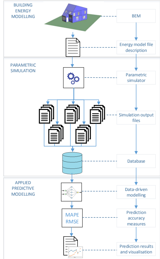
Figure 1: Methodology overview
