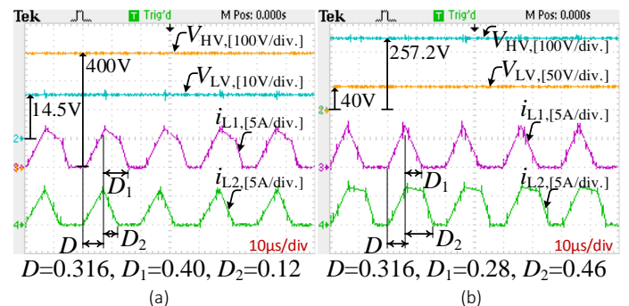
Fig. 15. Steady state operation of DCM in: (a) step-down and (b) step-up modes.
