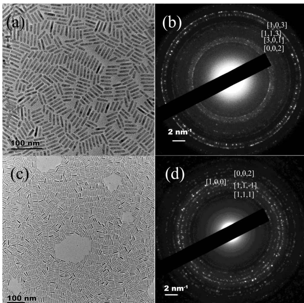
Fig. S2: \text{Cu}_7\text{S}_4 nanorods (b) electron diffraction of \text{Cu}_7\text{S}_4 and (c) \text{Ag}_2\text{S} nanorods and (d) electron diffraction of \text{Ag}_2\text{S}
