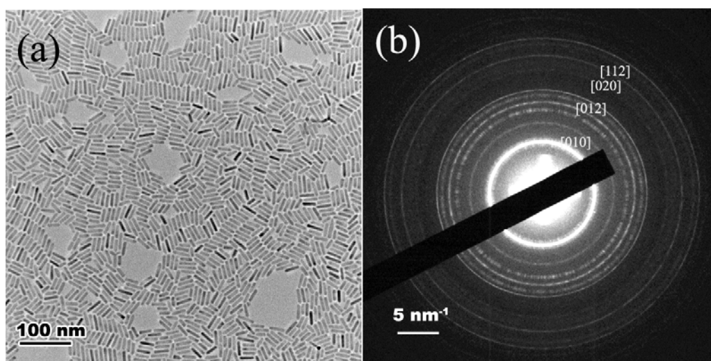
Fig. S1: (a) TEM image of CdS and (b) corresponding electron diffraction image.
