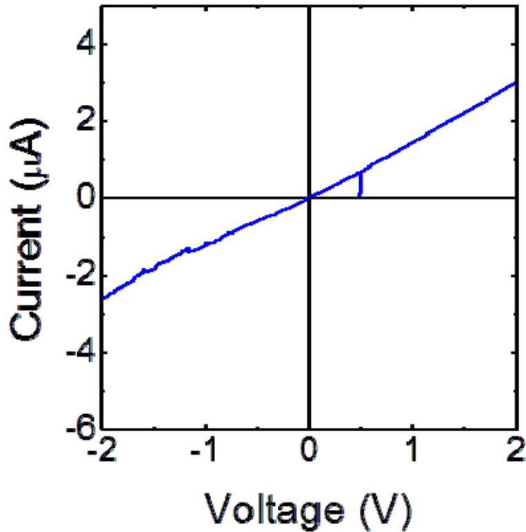
Fig. S5 Electrical measurements through spin exchanged \text{Ag}_2\text{S} as a thin deposit after sintering, exhibiting an ohmic response. The nanorod assembly was sintered to coalesce grains and removed organic contaminants from the surfactant employed to synthesize the nanorods and influence their assembly initially.
