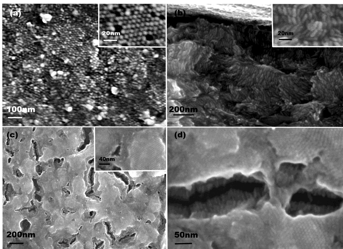
Fig S4: SEM images of (a) top down Ag 2 S assembly with inset clearly showing tips of nanorods, (b) cross section Ag 2 Se multilayer assembly with inset showing no shape change in the nanorods (c) top down Cu 7 S 4 assembly over a large scale with inset showing a HRSEM image of assembly (d) side on view of Cu 7 S 4 assembly with a view into the crack emphasising the multilayers of nanorods present within the assembly.
