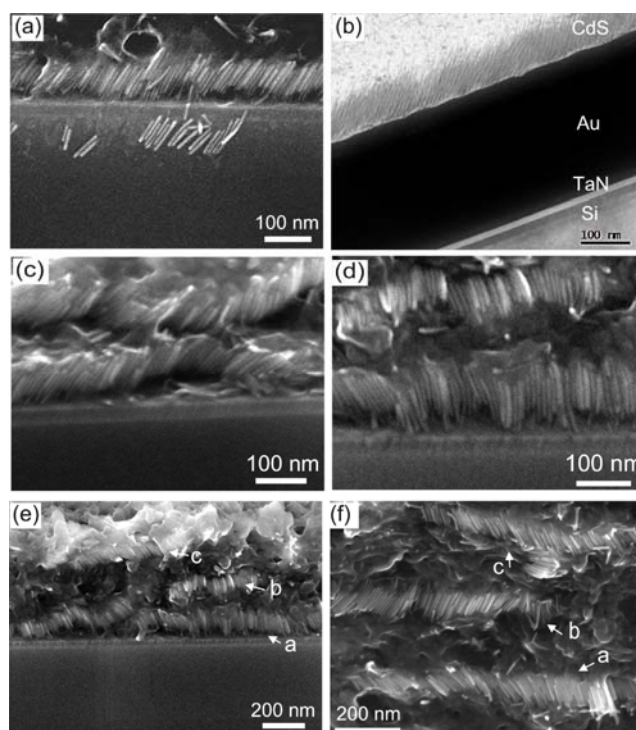
75 Fig. 2 (a) HRSEM image of CdS nanorod monolayer on Si/SiO 2 , after 300 seconds deposition (b) TEM image of FIB lift out sample of CdS monolayer on Au/TaN/Si substrate (300 seconds). (c-d) HRSEM images of bilayers formed after 600 s deposition. (e-f) HRSEM image of multilayer formation on Si/SiO 2 after 900 seconds deposition.
