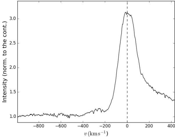
Fig. 3. CRILES spectrum of the Pa \beta line. Intensity is normalised to the continuum. Velocity is with respect to the LSR.
