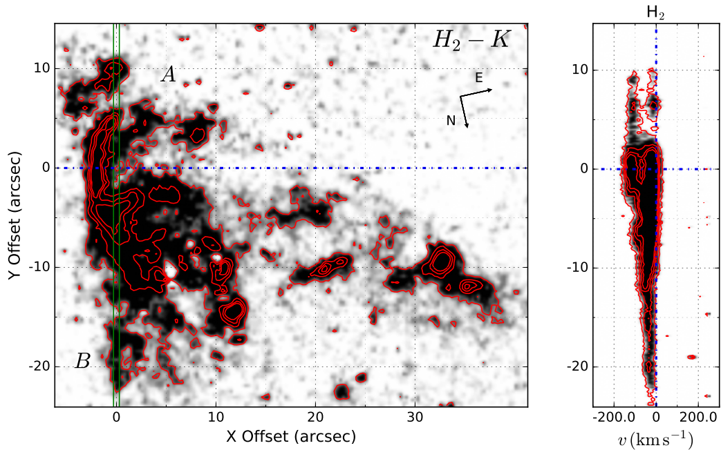
Fig. 7. PV diagram of slit 3. Left panel: SOFI H_2 - K continuum subtracted of the blue bow shock. Right panel: H_2 ( 2.12 \mu m ) line showing the two velocity components of the bow shock. Contours are from 3\sigma to 20\sigma in steps of 5\sigma . Radial velocities are with respect to LSR.
