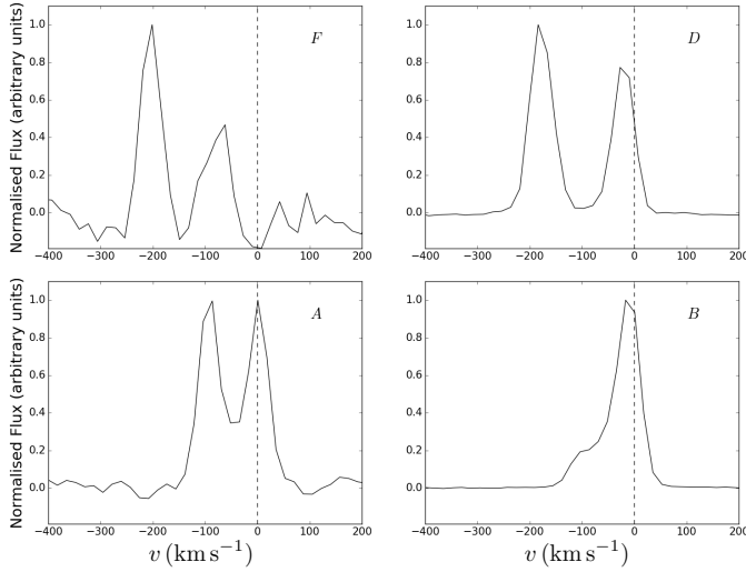
Fig. 8. H 2 1–0 S(1) line profiles for the investigated knots. Top left panel: F knot, top right panel: D knot, bottom left panel: A knot, and bottom right panel: B knot. Radial velocities are with respect to the LSR.
