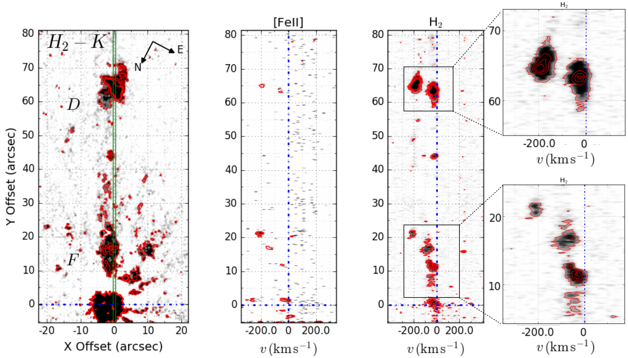
Fig. 6. PV diagram of slit 2. Left panel: SOFI H_2 - K continuum subtracted image (Caratti o Garatti et al. 2015a). Contours are from 3\sigma to 20\sigma in steps of 5\sigma . Middle panel: [Fe II] ( 1.644 \mu m ) line PV diagram tracing the atomic jet. Contours range from 3\sigma to 5\sigma in steps of 1\sigma . Right panel: H_2 ( 2.12 \mu m ) line PV diagram tracing the molecular jet. Contours are from 3\sigma to 20\sigma in steps of 5\sigma . Zoom-in panels of knots D (upper) and F (lower) with contours from 3\sigma to 80\sigma in steps of 20\sigma and from 3\sigma to 20\sigma in steps of 5\sigma , respectively. Radial velocities are in the LSR frame.
