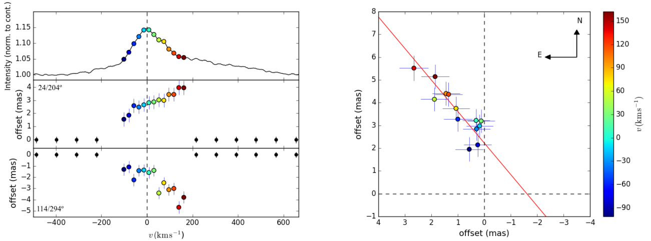
Fig. 5. Left panel: CRILES Br \alpha spectrum ( top panel ) along with the spectro-astrometric signal (in mas) detected in the jet parallel ( middle panel ) and perpendicular slit ( bottom panel ). The spectro-astrometric signal is continuum-corrected. Right panel: spectro-astrometric signal on the plane of the sky (north is up and east is to the left). The red line is the linear fit to the points giving a PA for the line-emitting region of 216 \pm 5^\circ . Error bars shown in both plots are 3\sigma . Velocities are colour coded and are the same in both panels.
