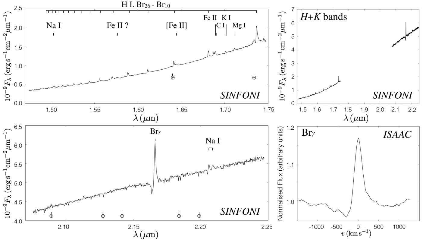
Fig. 2. Top left panel: H -band SINFONI spectrum on source. Detected lines and telluric features ( \oplus ) are labelled. Bottom left panel: K -band SINFONI spectrum on source. Top right panel: SED from the H and K spectra. Bottom right panel: zoom-in of the \text{Br}\gamma line of the ISAAC spectrum. Velocities are with respect to the local standard of rest (LSR).
