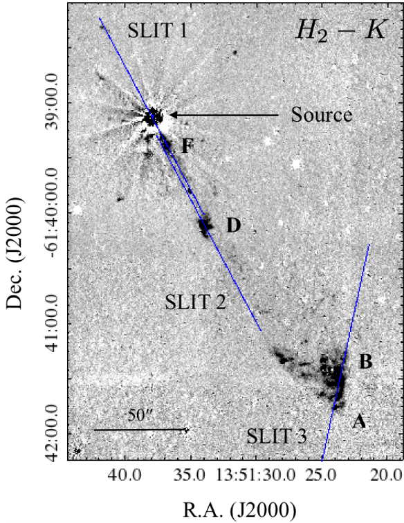
Fig. 1. SOFI 1 H_2 continuum-subtracted image of IRAS 13481-6124 showing the blue-shifted jet knots, bow shock, and driving source. Knot positions are labelled A, B, D, and F, following the notation of Caratti o Garatti et al. (2015a). ISAAC slit positions (blue) are labelled SLIT 1, 2, and 3 for convenience, and correspond to observations on the source, jet, and bow shock, respectively.
