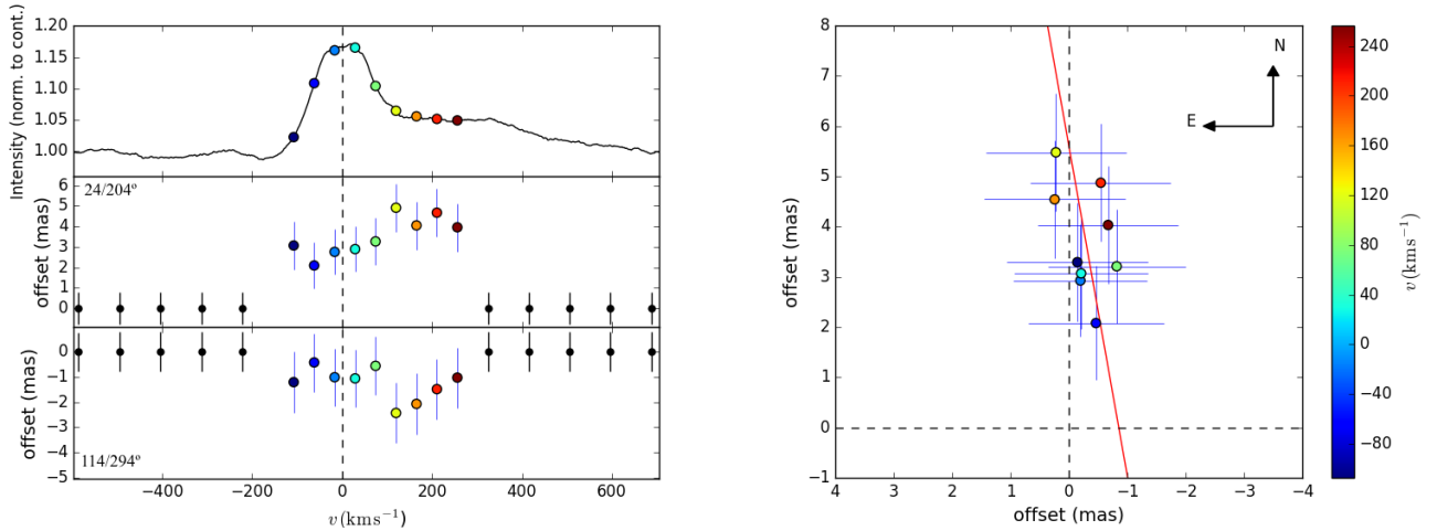
Fig. 4. Left panel: CRILES Br \gamma spectrum ( top panel ) along with the spectro-astrometric signal (in mas) detected in the jet parallel ( middle panel ) and perpendicular slit ( bottom panel ). The spectro-astrometric signal is continuum-corrected. Right panel: spectro-astrometric signal on the plane of the sky (north is up and east is to the left). The red line is the linear fit to the points giving a PA for the line-emitting region of 190 \pm 15^\circ . Error bars shown in both plots are 3\sigma . Velocities are colour coded and are the same in both panels.
