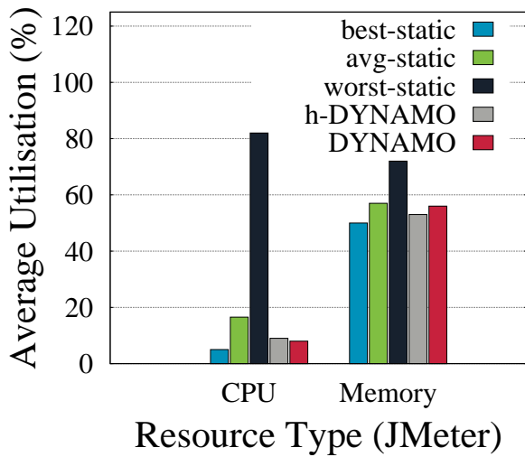
Figure 14: m-PetStore
