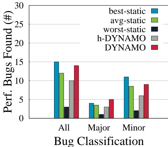
Figure 9: DaCapo
