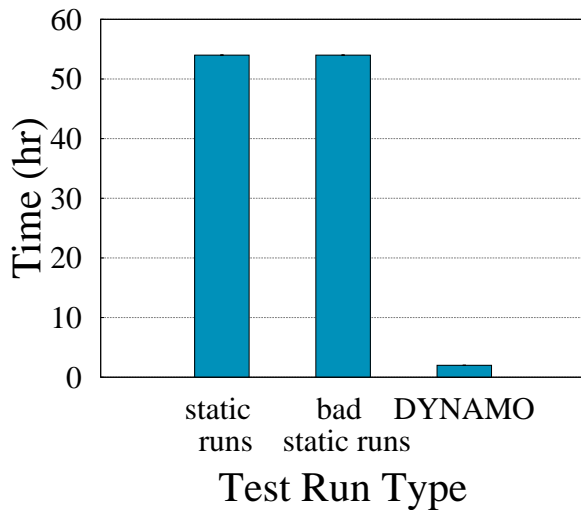
Figure 11: m-PetStore
