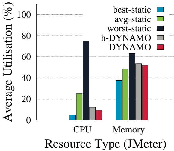
Figure 13: PetStore
