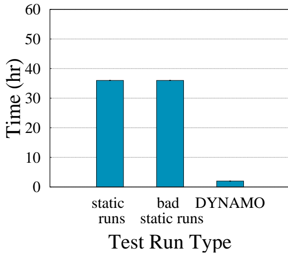
Figure 10: PetStore
