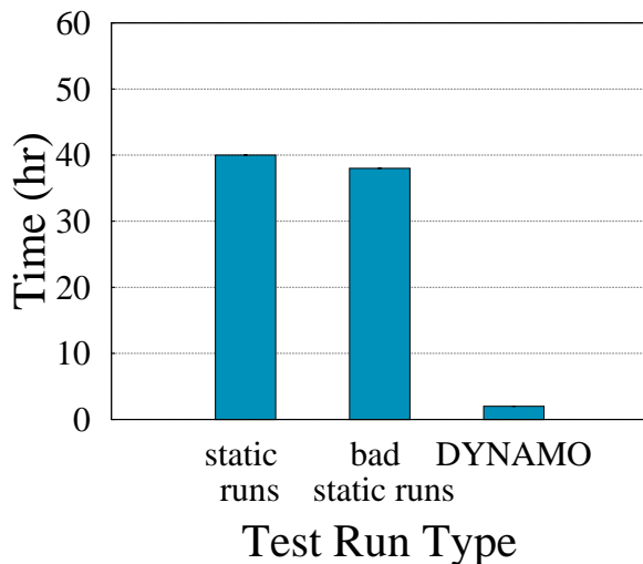
Figure 12: DaCapo
