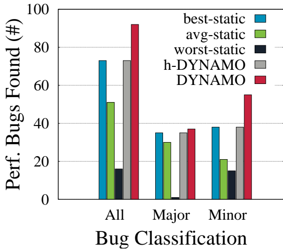
Figure 7: PetStore
