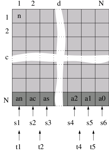
Fig. 1. Representation of the Chebyshev discretization for a system with s delays \tau_1 < \tau_2 < \dots < \tau_{s-1} < \tau_s . In the general case, the delays do not match exactly the grid and, thus, an interpolation between consecutive nodes of the grid is required.
