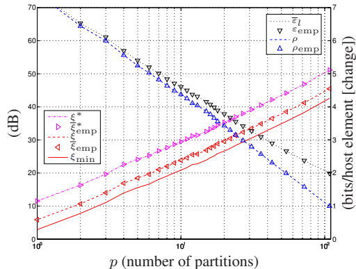
Fig. 1. Performance of permutation coding using adaptive partitioning. Lines are theoretical predictions and symbols are empirical results. Host: 512 \times 512 grayscale Lena (8 bpp), spatial domain.
