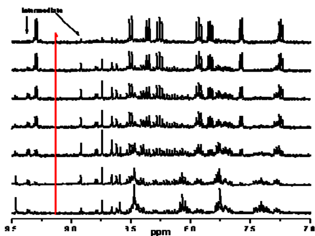
Fig. 5. Irradiation of N2 isomer of [\text{Ru}(\text{bpy})_2(\text{Hpztr})]^{2+} in acetonitrile with \text{CF}_3\text{CO}_2\text{H}
