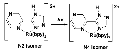
Fig. 2 Reversible N2-N4 isomerisation observed for compound 2H .
