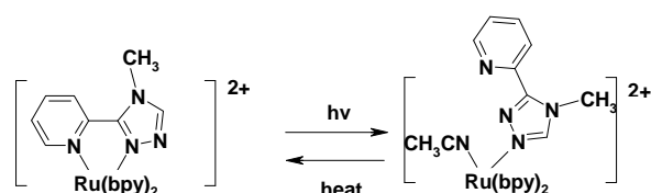
Fig. 6 Photo- and thermally induced coordination changes for [\text{Ru}(\text{bpy})_2(\text{L}-\text{L}') ]^{2+} where L-L' is 4-methyl-3-(pyridine-2-yl)-1,2,4-triazole
