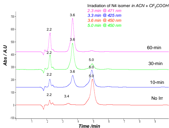
Figure 4. HPLC trace following the irradiation of the N4 isomer in \text{CH}_3\text{CN} with \text{CF}_3\text{CO}_2\text{H} (Mobile phase \text{CH}_3\text{CN}:\text{H}_2\text{O}:\text{CH}_3\text{OH} with volume ratio 75:20:5 0.12 M \text{KNO}_3 ). Flow rate: 2.0\text{ cm}^3\text{ min}^{-1} ; detection wavelength: 430 nm, @ 20^\circ\text{C}
