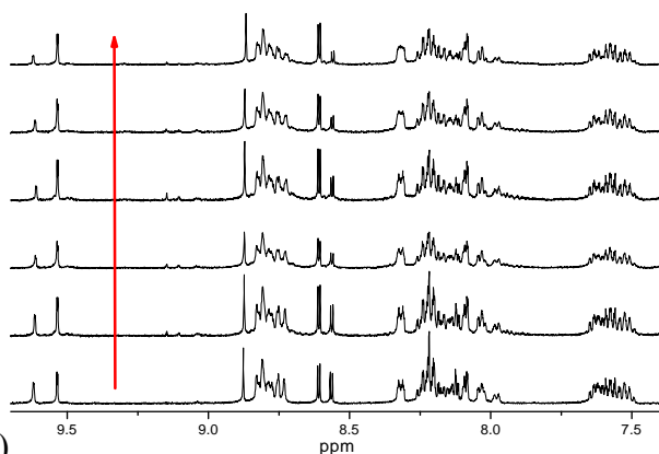
Fig. 8. a) Irradiation of the N2 isomer of [Ru(bpy) 2 (Hpztr)] 2+ ( 1H ) in acetone with CF 3 CO 2 H. (b) Irradiation of a 1:1 mixture of the N2 and N4 isomer of [Ru(bpy) 2 (Hpztr)] 2+ ( 1H ) in acetone with CF 3 CO 2 H. Spectra run from bottom to top in each case.
