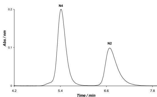
Fig. 3 HPLC trace of N2 and N4 isomers of 1 . Mobile phase \text{CH}_3\text{CN} : \text{H}_2\text{O} : \text{CH}_3\text{OH} with volume ratio 75:20:5, 0.12 M \text{KNO}_3 Flow rate: 2.0 \text{cm}^3 \text{min}^{-1} ; detection wavelength: 430 nm, @ 20 ^\circ\text{C} .
