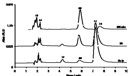
Figure 7 HPLC assessment of the photoisomerisation of N2 isomer of 1H in acetone in the presence of CF 3 COOH.
