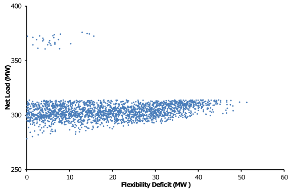
Fig. 9. Net load during periods of insufficient flexibility
