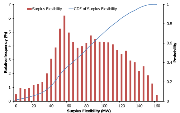
Fig. 8. Relative frequency and cumulative probability distribution of surplus flexibility
