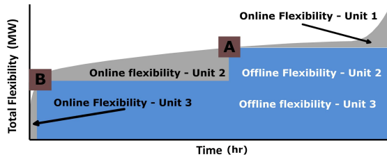
Fig. 3. Available flexibility series
