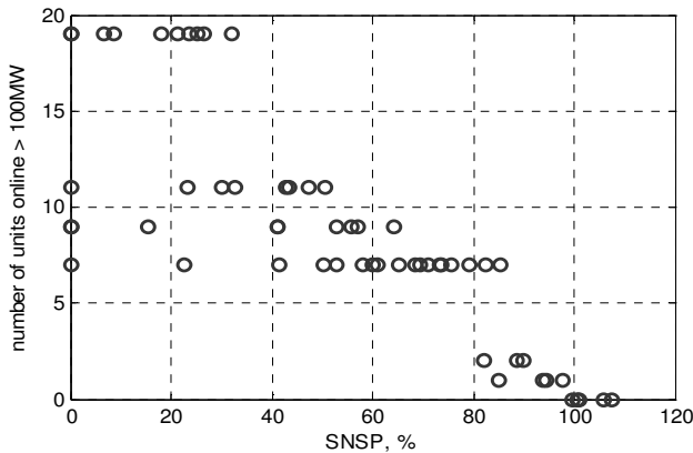
Fig. 4 – Number of conventional synchronous plants > 100 MW online with respect to instantaneous SNSP
