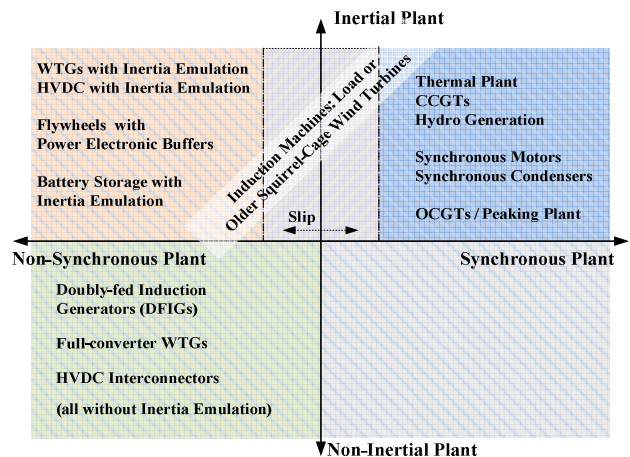
Fig. 1- Classification of power generation sources according to whether they are synchronized to the system and/or provide inertia
