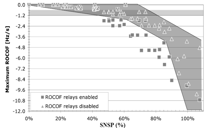
Fig. 7 – Corresponding impact of voltage disturbances (35% dip of nominal voltage) on maximum ROCOF
