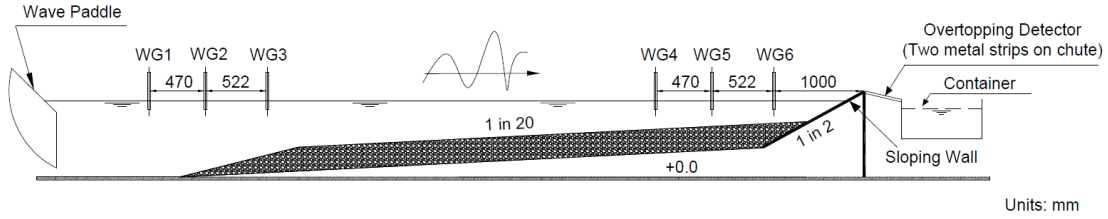
Figure 1. Schematic of the experimental set-up (adapted from Salauddin and Pearson, 2020)
