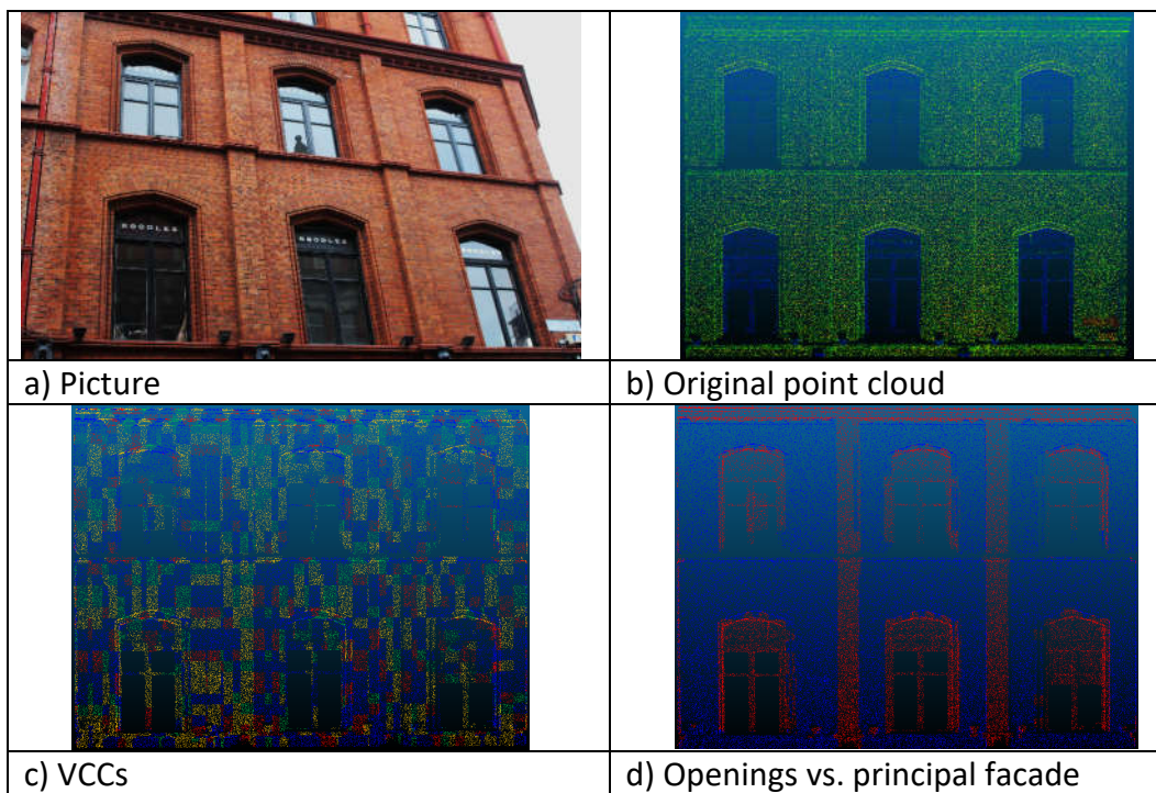
Fig. 7. Recess vs. principal facade display, failure on vertical recess detection; 71 Grafton (Building 5)
