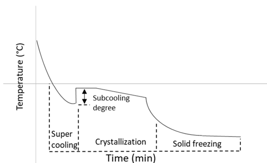
Figure 10. Schematic of typical freezing curve.
