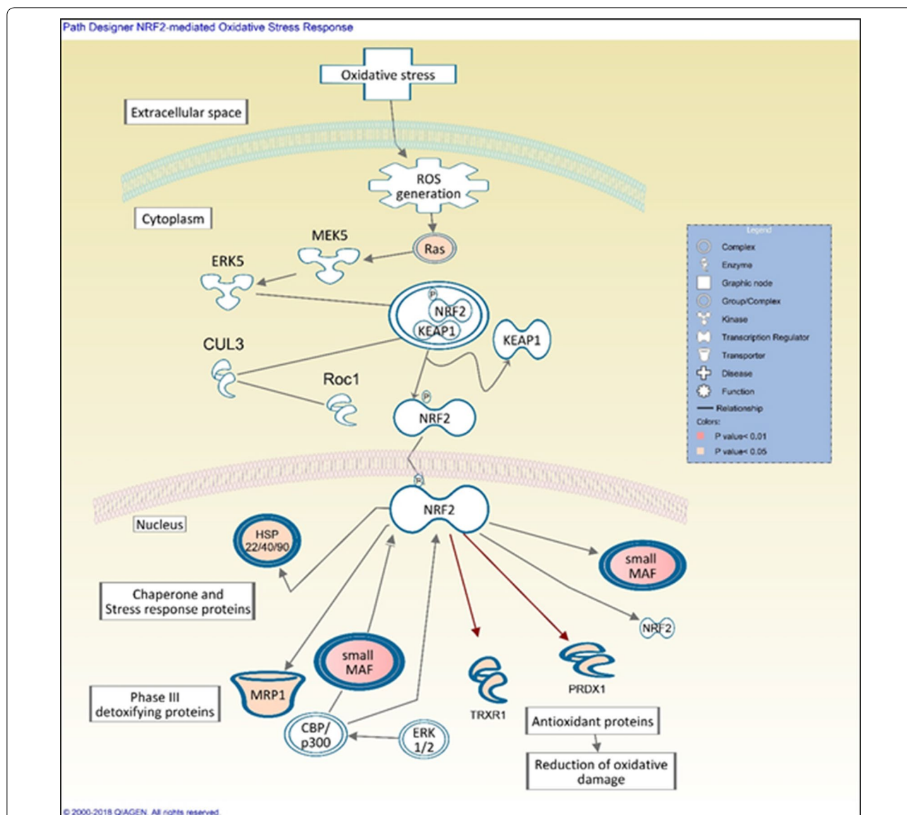
Fig. 4 Gene expression analysis by IPA software ( FC \geq 1.5 and p value < 0.001 ) showing nuclear factor erythroid 2-related factor 2 (NRF2) oxidative stress response path design activated in NR8383 cells after exposure to \frac{1}{4} IC_{50} of NM403 for 4 h. Only upregulated genes implicated in this pathway are shown. Double bold line means that we have a complex
