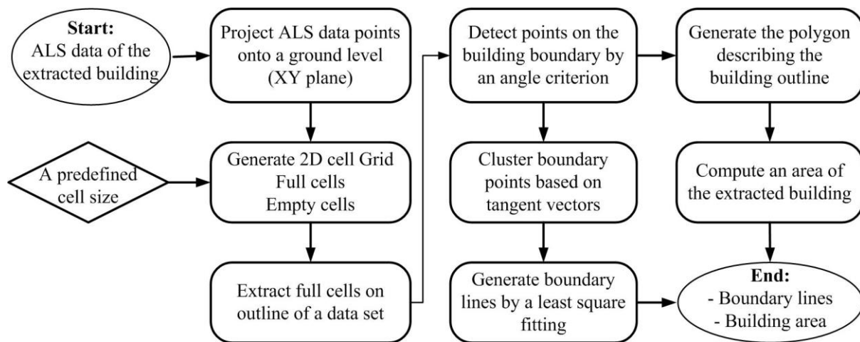
Figure 8. Workflow to generate boundary lines of extracted buildings
