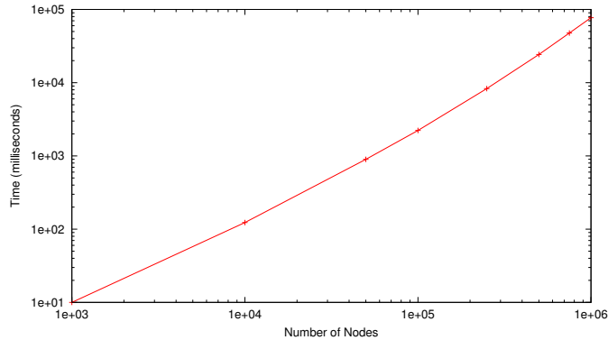
Figure 8: Plot of running time in milliseconds against number of nodes, for the proposed dynamic community finding method ( \theta = 0.5 ) on synthetic graphs of increasing size from 1,000 to 1 million nodes.
