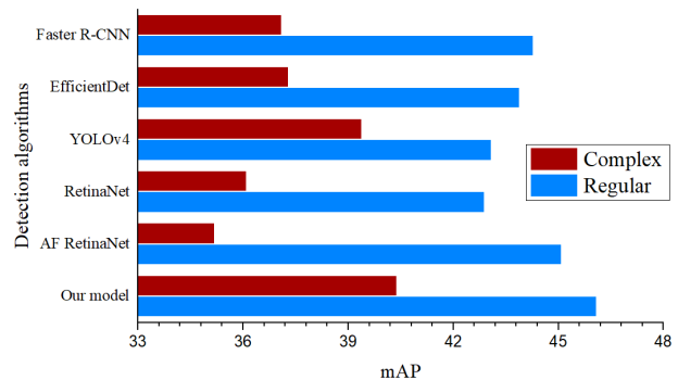
Fig. 13. Detection performance for images with different scenarios.
