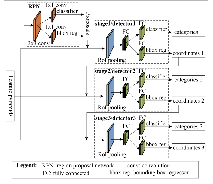
Fig. 5. The procedure of three-stage detection with three sequential and homogeneous detectors.
