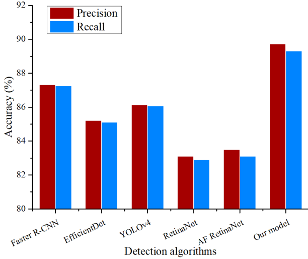
Fig. 9. The precision performance evaluating the number of occupants being correctly detected.
