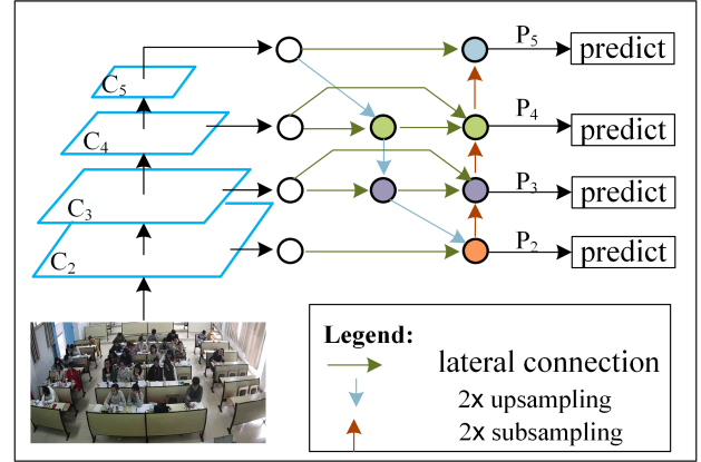
Fig. 4. The feature network of constructing feature pyramids with bidirectional cross-scale connections.
