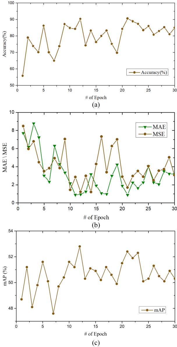
Fig. 6. Convergence curves for the deep learning model training (a) accuracy results, (b) MAE and MSE results, and (c) mAP results.
