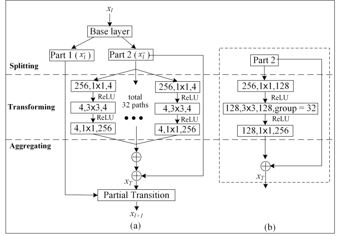
Fig. 3. (a) a building block of DCNN with cardinality = 32; (b) a building block of DCNN with grouped convolutions.
