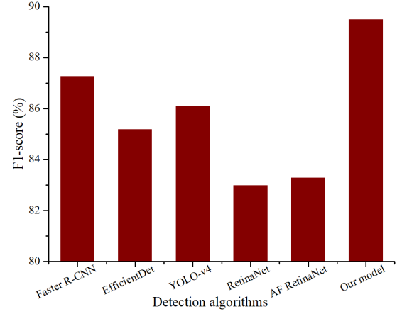
Fig. 10. Detection performance of all detection models in F1 score.
