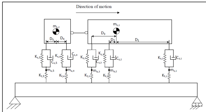
Figure 9. Truck-Trailer Model.
