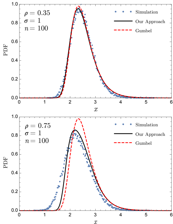
Fig. 3. The p.d.f. of the Gumbel distribution (dashed red) and given by (15) (solid black) together with the results of numerical simulations (blue dots) for different values of the correlation coefficient \rho .
