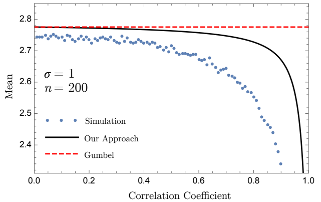
Fig. 4. The mean of RV (5) for n = 200 as a function of \rho . The black solid curve is the mean obtained from p.d.f. (15). The red dashed line is due to (8). Blue dots represent the results of the numerical simulation.
