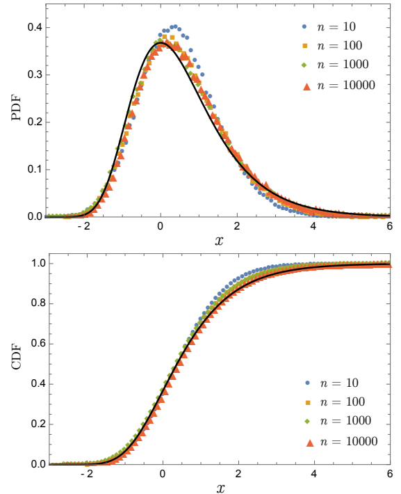
Fig. 2. The p.d.f. \Psi'_n(x) and c.d.f. \Psi_n(x) of the Gumbel distribution (black solid lines) versus numerical simulations of the RV (5) for different values of n . The samples are scaled so that a_n = 0 and b_n = 1 .
