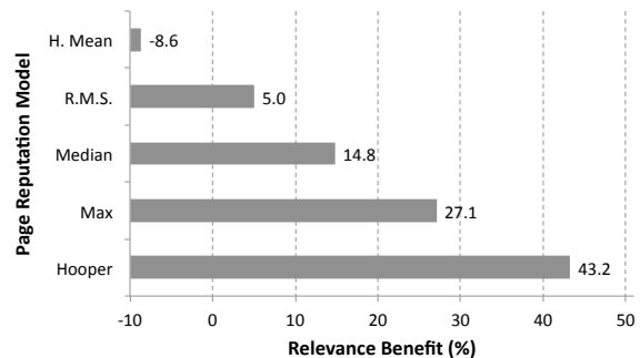
Fig. 5. Median relevance benefit across weights per page reputation model.
