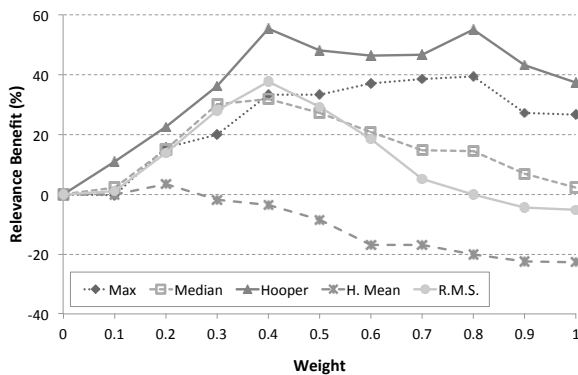
Fig. 4. Relevance benefit for page reputation models vs. weight.
