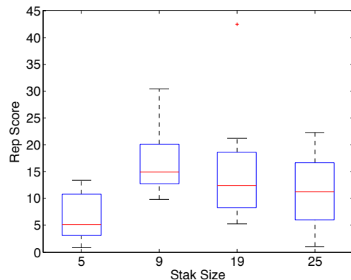
Fig. 3. User reputation score per user, per stak.
