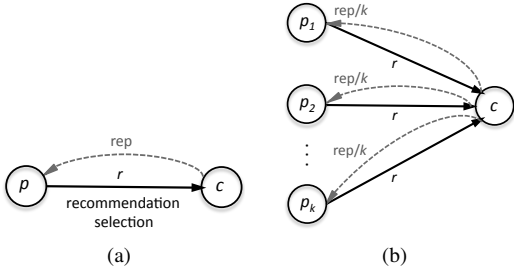
Fig. 2. Collaboration and reputation: (a) the consumer c selects result r , which has been recommended based on the producer p 's previous activity, so that c confers some unit of reputation ( rep ) on p . (b) The consumer c selects a result r that has been produced by several producers, p_1, \dots, p_k ; reputation is shared amongst these producers with each user receiving an equal share of rep/k units of reputation.
