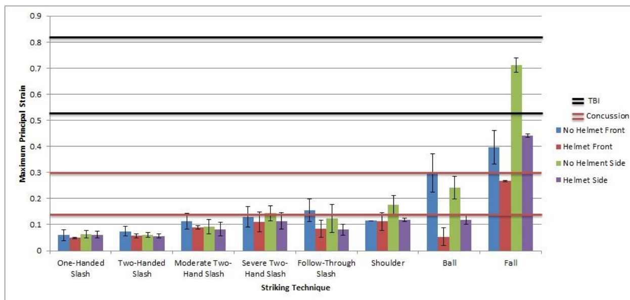
Fig. 3. Maximum principal strain across all impact conditions. The two black lines represent the reported range of reported traumatic brain injury (TBI) (Doorly, 2007; Doorly and Gilchrist, 2006; Post et al., 2015b) and the two red lines represent the range of reported concussions (Kendall, 2016; Oeur et al., 2015; Rousseau, 2014; Zanetti et al., 2013).
