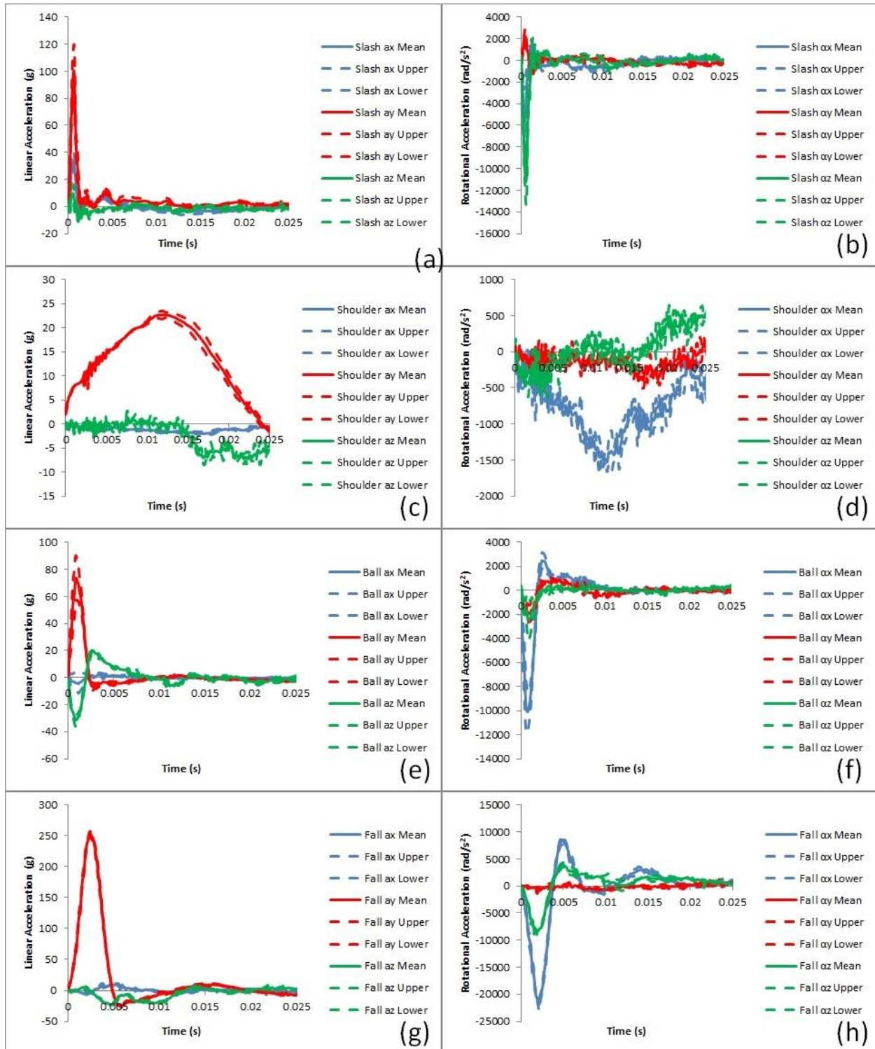
Fig. 1. Mean six degrees of freedom linear and rotational traces from a Hybrid III headform for slashing, shoulder collisions, ball impacts and falls (Clark and Hoshizaki, 2016): (a) Linear acceleration traces for slashing, (b) Rotational acceleration traces for slashing, (c) Linear acceleration traces for shoulder collisions, (d) Rotational acceleration traces for shoulder collisions, (e) Linear acceleration traces for ball impacts, (f) Rotational acceleration traces for ball impacts, (g) Linear acceleration traces for falls, (h) Rotational acceleration traces for falls.
