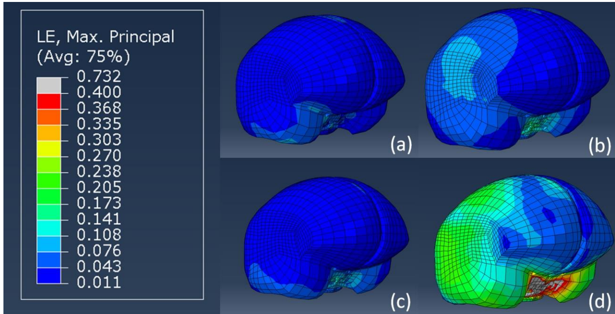
Fig. 2. Strain distribution at maximum (only the cerebrum of the brain model is shown) for one case of: (a) slashing, (b) shoulder collision, (c) ball impact and (d) fall.
