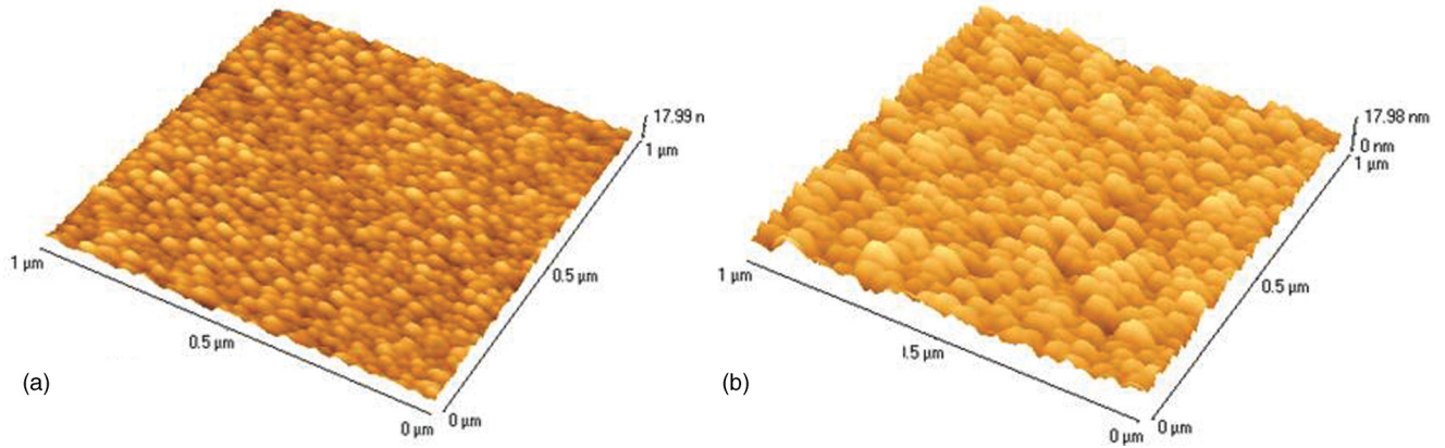
FIG. 4. (Color online) AFM topographical morphology of (a) undoped and (b) 5% Cr-doped sputtered-deposited \text{TiO}_2 coating.
