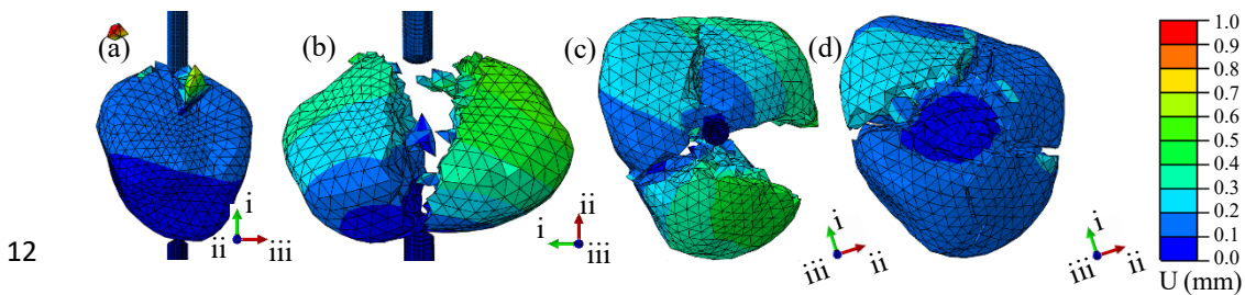
12 13 Fig. 10 Three types of fracture patterns due to rotational point loading: (a) chipping; (b) 14 two main fragments splitting; (c) three main fragments splitting; (d) platen load towards 15 minimum dimension (i, ii and iii denote maximum, median and minimum principal 16 dimensions, respectively, of the intact LBS particle before compressed). Coloured by 17 the scalar displacement, U.
