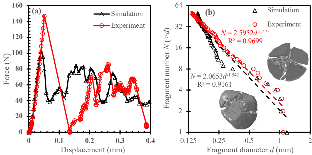
2 Fig. 6 Comparison of results for simulated and experimental 1D compression tests of 3 single particle using flat platen: (a) Load-displacement curves; (b) Fractal distribution 4 of fragment volume-equivalent sizes with two snapshots for the simulation (the left) 5 and experiment (the right) at 0.135 mm displacement
