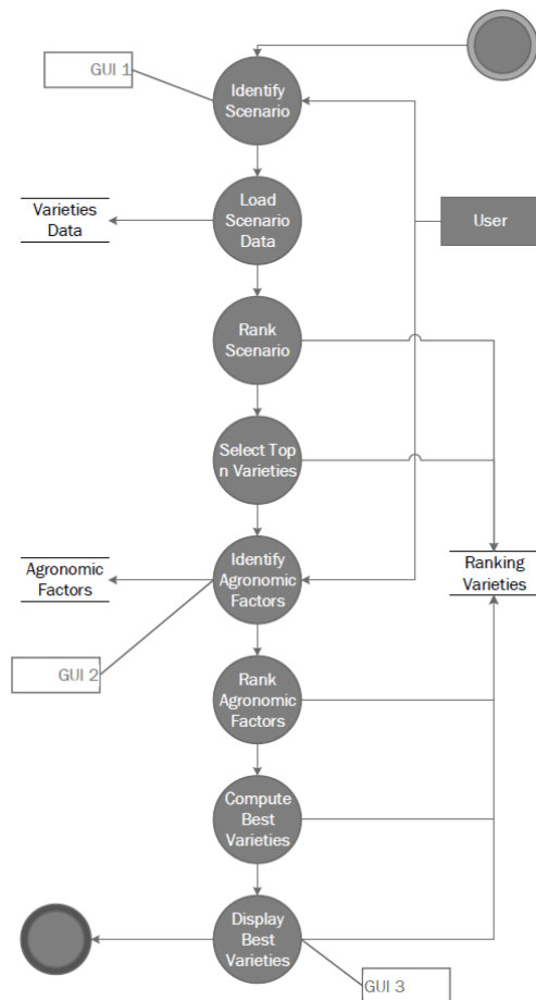
Figure 2. Data flow diagram expressing the different steps on the process of variety selection.
