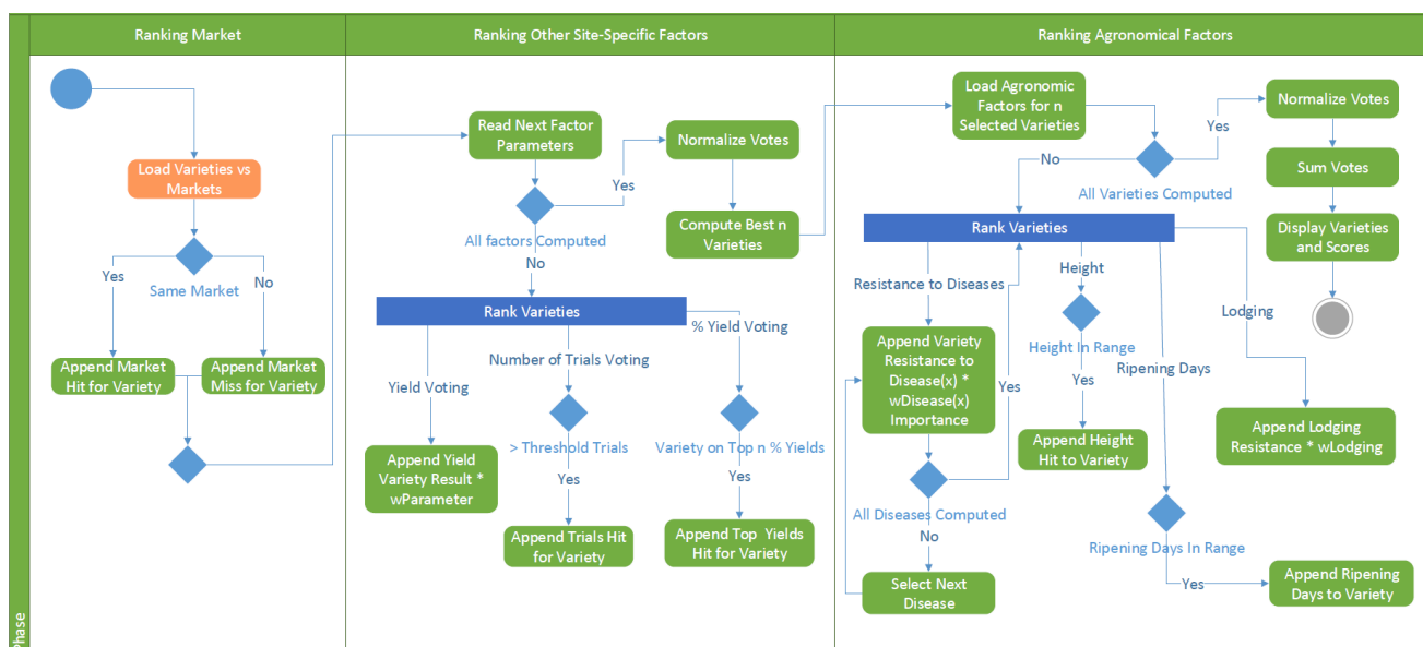
Figure 5. Activity diagram showing the different phases of the ranking process where varieties votes are computed accordingly to site-specific and importance of agronomical traits selected by the user.
