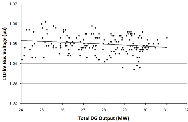
Fig. 4. Nose of PV Curve for 110 kV BSP bus with fixed 0.95 power factors
