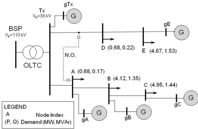
Fig. 1. 38 kV 5 bus radial distribution network diagram (max. load level)
