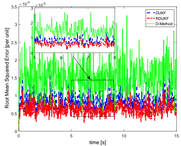
Fig. 4: RMSE of DUKF, RDUKF and D-method with large measurement noise in the IEEE 39-bus system, where the variance is changed from 10^{-6} to 10^{-4} .
