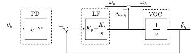
Fig. 4: Block diagram of the SRF-PLL.
