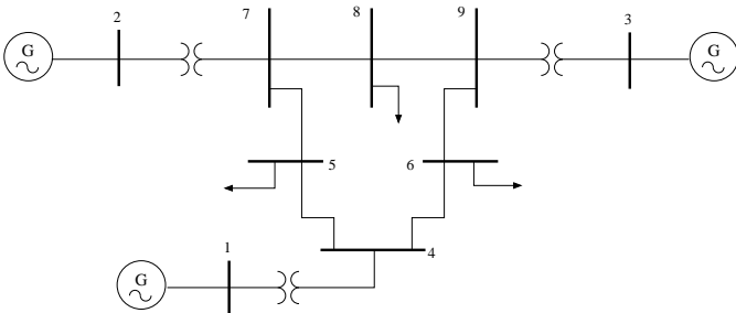
Fig. 3: WSCC 9-bus system.
