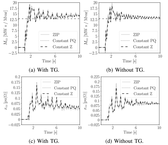
Fig. 6: 50% increase of load connected to bus 6. Impact of load model and TGs.
