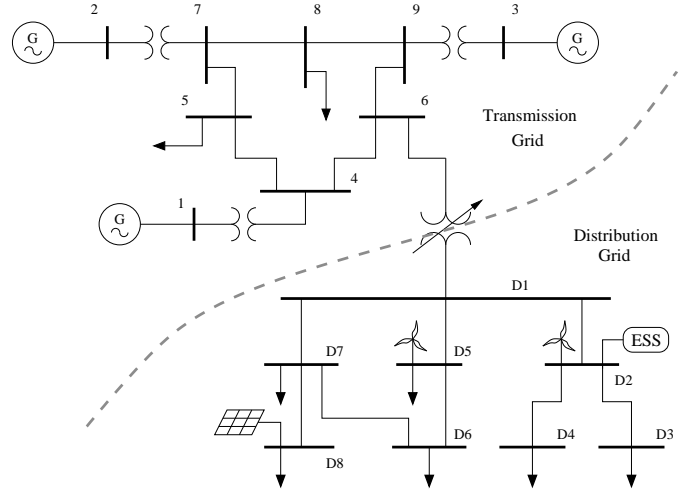
Fig. 8: WSCC 9-bus system modified to include the VPP.
