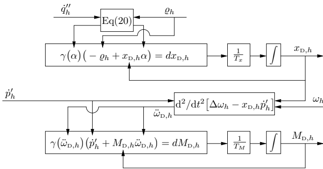
Fig. 2: Real-time loop for the proposed inertia estimator.
