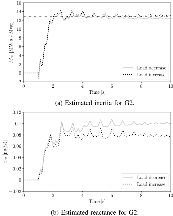
Fig. 5: 20% variation of load connected to bus 6.
