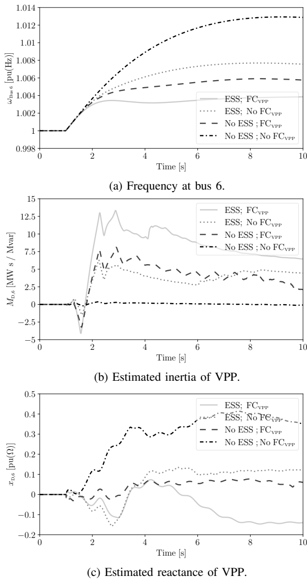
Fig. 9: 20% decrease of load connected to bus 5.
