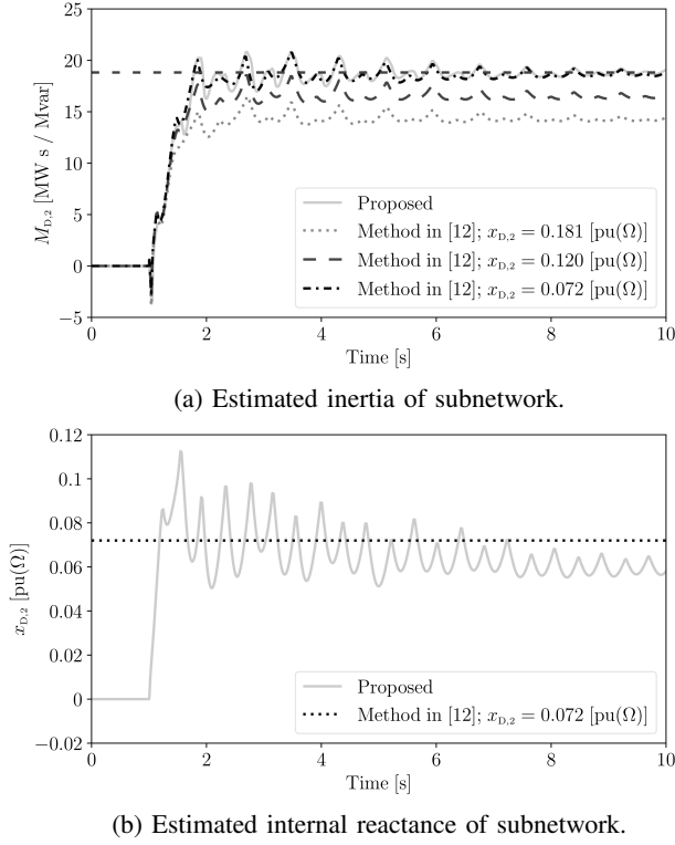
Fig. 7: 20% increase of load connected to bus 8.
