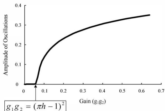
Figure 5. Amplitude of oscillation as a function of gain ( g_1g_2 ) for a value of h = 0.4 (system is not self-oscillatory). The curve is derived by simulation of the system shown in Fig. 1.
