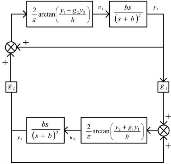
Figure 1. The basic system considered. +/- coupling has g_1 = g_2 > 0 ; +/- coupling has g_1 = -g_2 < 0 .
