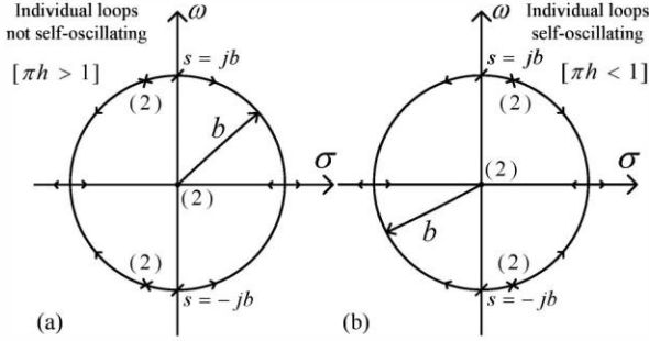
Figure 3. (a) shows root motion for non-oscillatory system ( \pi h > 1 ). As the gain is increased, the system begins to oscillate when a pair of complex conjugate roots cross the imaginary axis. The frequency of oscillation decreases with increasing gain. (b) is for a self-oscillatory system ( \pi h < 1 ). As the gain increases one frequency of oscillation increases slightly then disappears as the corresponding complex pair of roots enters the left half plane. The other complex pair move to the right, with frequency decreasing.
