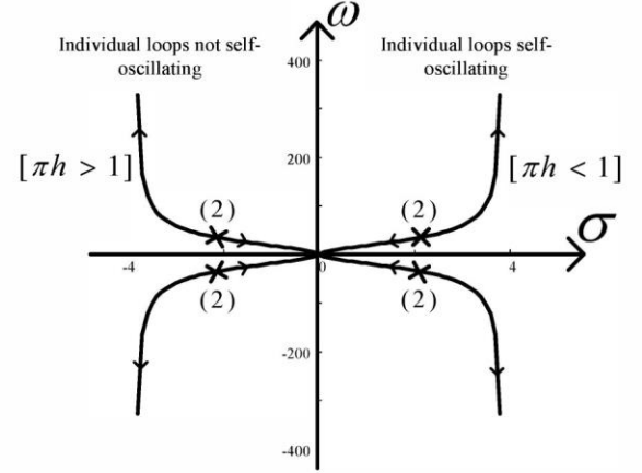
Figure 4. Root locus sketches for individual loops self-oscillating (right half plane) and not self-oscillating (left half plane).
