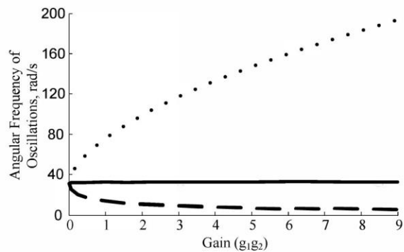
Figure 7. The angular frequencies of oscillation of y_1 as a function of gain ( g_1g_2 ) derived by simulating the system shown in Fig. 1, for the “+/-” case, with h = 0.3 (system self-oscillatory). The geometric mean of the two frequencies, which remains almost constant, is also included.
