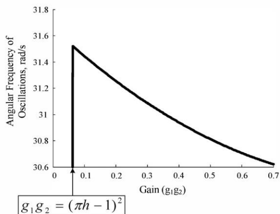
Figure 6. The angular frequency of oscillation of y_1 as a function of gain ( g_1g_2 ) derived by simulating the system shown in Fig. 1 for the “+/-” case. The loops are not self-oscillatory, with h = 0.4 .
