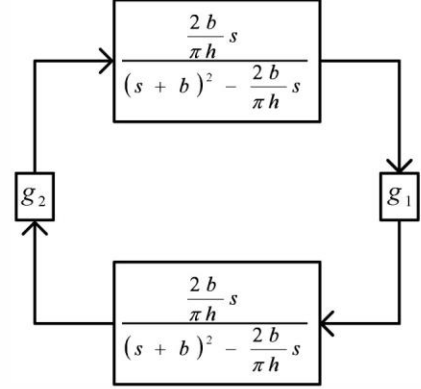
Figure 2. Small signal (linearized) equivalent of Fig. 1.
