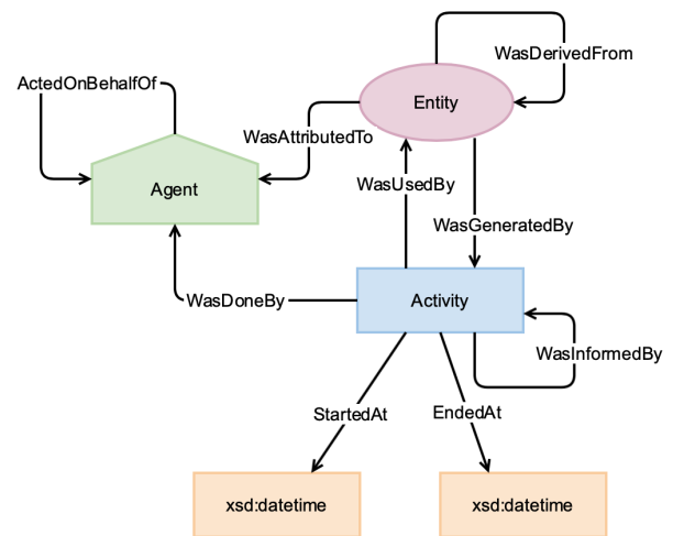
Figure 1: W3C's Prov-O (PROV-O: The PROV Ontology (2013)) Ontology for Provenance Management.
