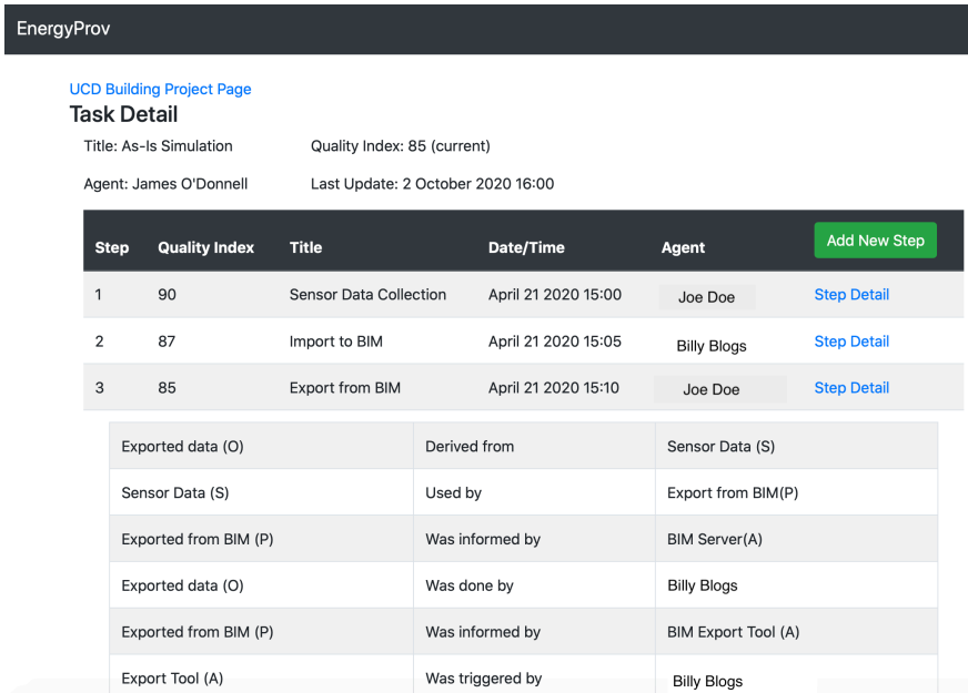
Figure 3: Interface that describes a simulation step, including a summary steps taken to complete the task. Each step can be viewed in detail by clicking on a row.
