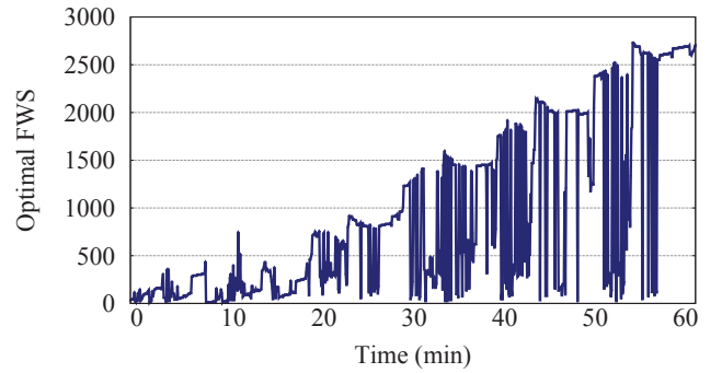
Fig. 6. sGC Eclipse-100MB: FWS vs. Time
