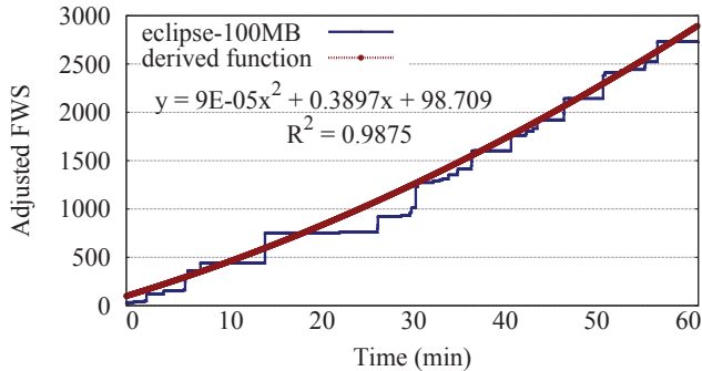
Fig. 9. sGC Eclipse-100: Derived FWS Trending Function
