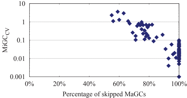
Fig. 17. Comparison of Skipped MaGC vs. Experienced MiGC_{CV}
