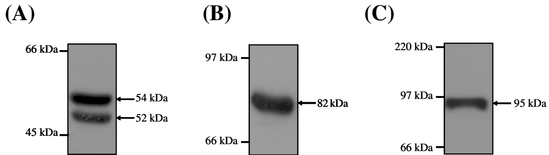
Figure 2: Expression of WT1, Sp1 and Egr1 proteins in HEL 92.1.7 cells. Immunoblot analysis of WT1 (Panel A), Egr1 (Panel B) and Sp1 (Panel C) expression in HEL cells (60 \mu g whole cell protein per lane). The positions of the molecular size markers (kDa) are indicated to the left, while the sizes of WT1, Sp1 and Egr1 are indicated to the right of the panels, respectively.
