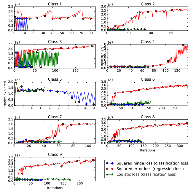
Fig. 5. Malware: Number of nodes explored by different loss functions (blue for hingloss, green for logreg, red for SqLoss) for all 9 classes.
