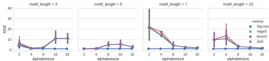
Fig. 1. Average MSE across 5 runs, comparing the impact of varying data generation parameters (alphabet size, motif length) on 4 regression methods. SqLoss has the lowest MSE across all data generation scenarios.
