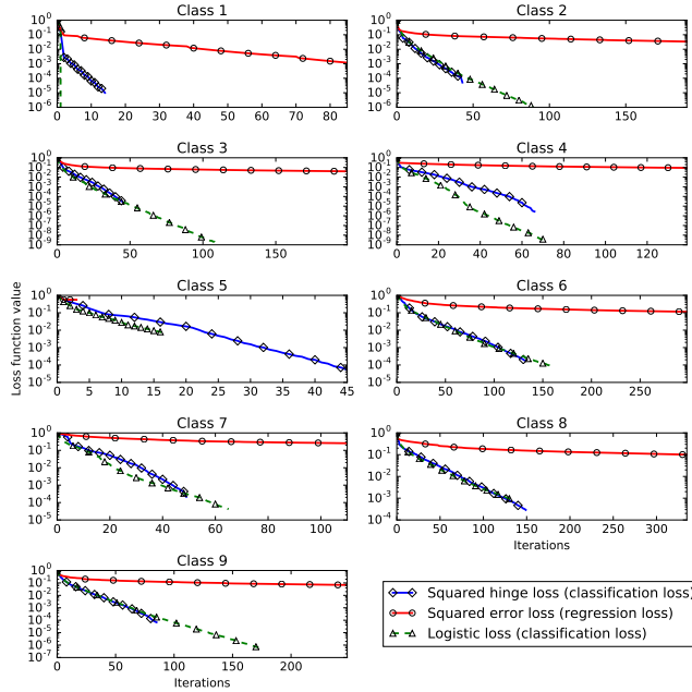
Fig. 4. Malware: Comparison of loss functions per iteration for all 9 classes. Blue for squared hinge loss, green for logistic regression and red for SqLoss.
