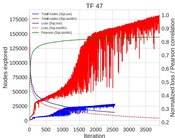
Fig. 3. TF-DNA: Loss and explored nodes per iteration, w/o wildcard for protein TF47. In blue SqLoss, in red SqLossWc. Pearson correlation (green) for SqLossWc.
