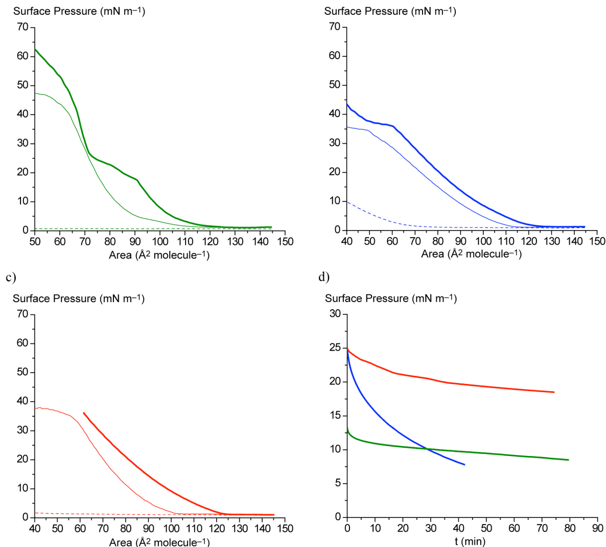
Fig. 6 Chain length dependence of the isotherm plots of Langmuir monolayers of complexes 3 (a), 4 (b), and 5 (c), different alkoxy substituents are represented by dashed (OC 6 H 13 ), solid (OC 12 H 25 ), or bold lines (OC 18 H 37 ); (d) film stability over time of monolayers composed of 3c (green), 4c (blue), and 5c (red).
