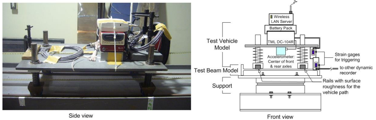
Fig. 5. Experimental vehicle.
