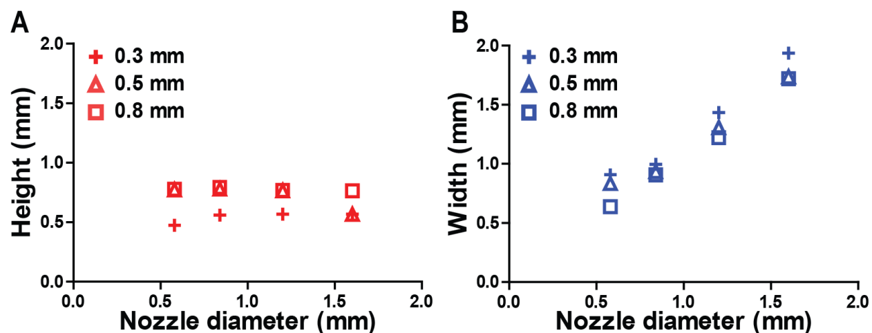
Figure 4. (A) Height and (B) width of gelatin alginate hydrogels printed into 60 mM CaCl 2 using nozzle distances of 0.3, 0.5, and 0.8 mm, an extrusion rate of 12 mm/s, and nozzle diameters of 0.58, 0.84, 1.20, and 1.60 mm.
