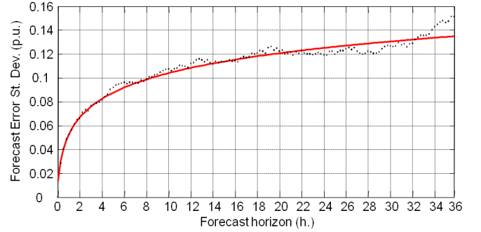
Fig 1. Normalized standard deviation of wind power forecast error for 12 GW installed capacity versus forecast horizon (Source: Netherlands, AVDE tool with data from the atmospheric model HIRLAM [10]). Solid line is a curve fitting.
