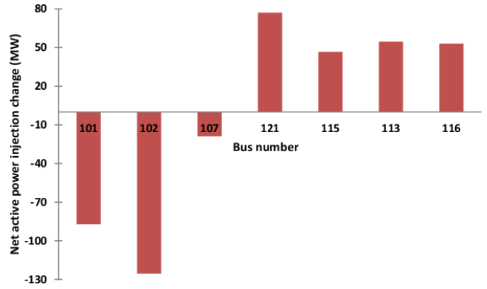
Fig. 3. Changes in net active power injections (generation minus load) due to N-1 security constraints within unit commitment
