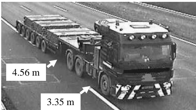
(a) GVW=100.1 t, wheelbase=16.2 m (carrying crane ballast).
