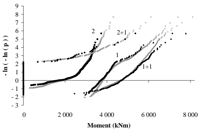
(a) Mid-span moment, simply supported
