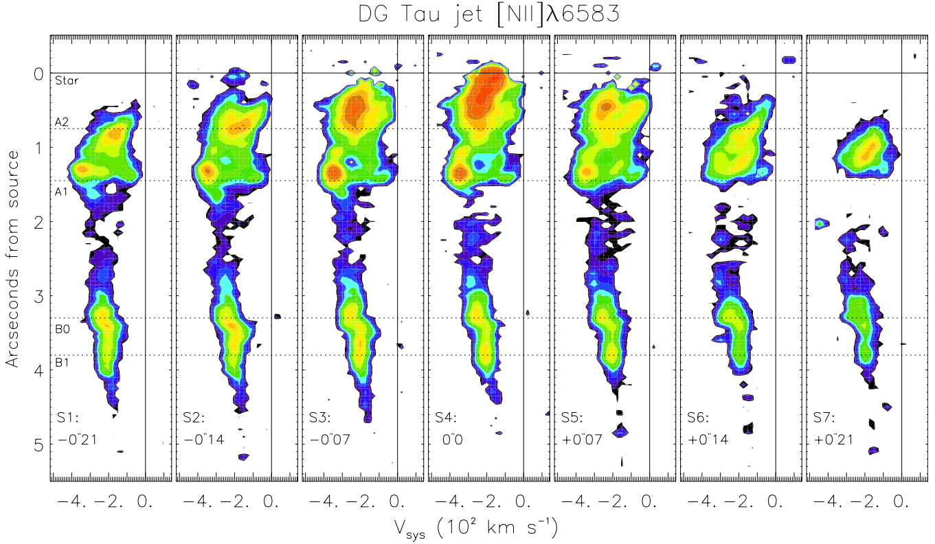
Fig. 3. Same as Fig. 1, but for [N II] \lambda 6583.
