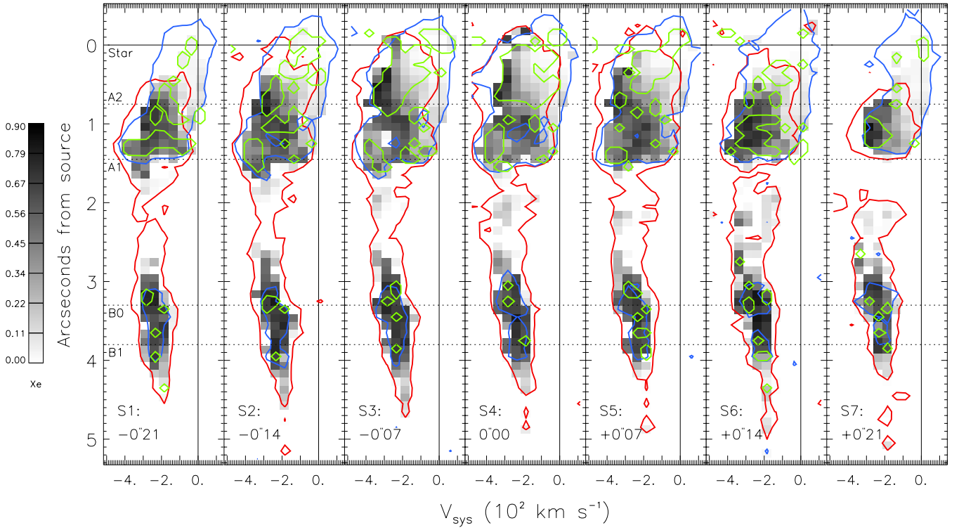
Fig. 8. Position-velocity diagrams of the ionisation fraction x_e . Contours: blue – [O I] \lambda 6363 at 3\sigma ; red – [N II] \lambda 6583 at 3\sigma ; green – high density limit for the [S II]31/16 ratio. Where only [O I] ([N II]) is above 3\sigma , x_e is an upper (lower) limit. Inside the HDL regions x_e is determined with the HDL-BE procedure (cf. Sect. 2.2).
