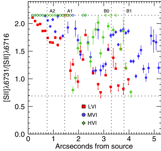
Fig. 16. 1D profile of the [S\ II]_{31/16} ratio along the flow, derived from integration of the line surface brightness across the jet and over each velocity interval. Horizontal dashed lines indicate upper and lower density limits on validity of the ratio as a n_e diagnostic. Empty symbols mark positions and velocities for which the modified BE-technique has been applied. Upper and lower limits arise when one of the lines is undetected, and so its flux has been set to 3\sigma .
