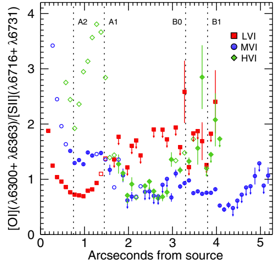
Fig. 18. Same as Fig. 16 for the [O\ I]/[S\ II] line ratio. Due to the prominence of [O\ I] emission over the [S\ II] lines close to the star, a few points are off the scale. Their values are: 6.58 at 0'.175 , for the MVI, and 12.10, 14.49, 9.54 and 4.99 at 0'.175 , 0'.275 , 0'.375 and 0'.475 , respectively, for the HVI.
