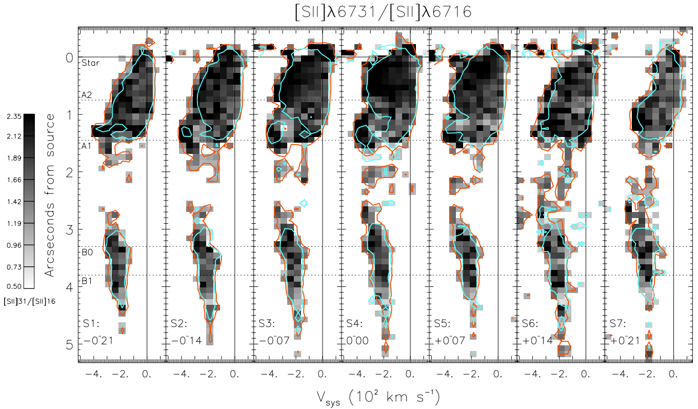
Fig. 4. Position-velocity plots of the [S II] \lambda 6731/[S II] \lambda 6716 line ratio in linear greyscale. Cyan and orange contours indicate the [S II] \lambda 6716 and [S II] \lambda 6731 emission at 3\sigma , respectively. Where only one of the two lines is above the 3\sigma threshold the upper/lower limit of the line ratio is reported.
