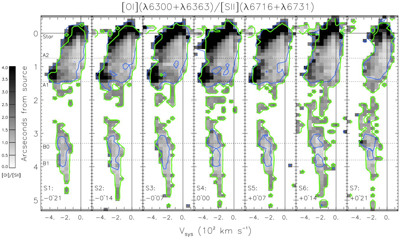
Fig. 6. Same as Fig. 4 for [\text{OI}](\lambda 6300 + \lambda 6363) / [\text{SII}](\lambda 6716 + \lambda 6731) line ratio. Blue and green contours indicate [\text{OI}]\lambda 6363 and the [\text{SII}]\lambda 6731 + \lambda 6716 emission at 3\sigma respectively.
