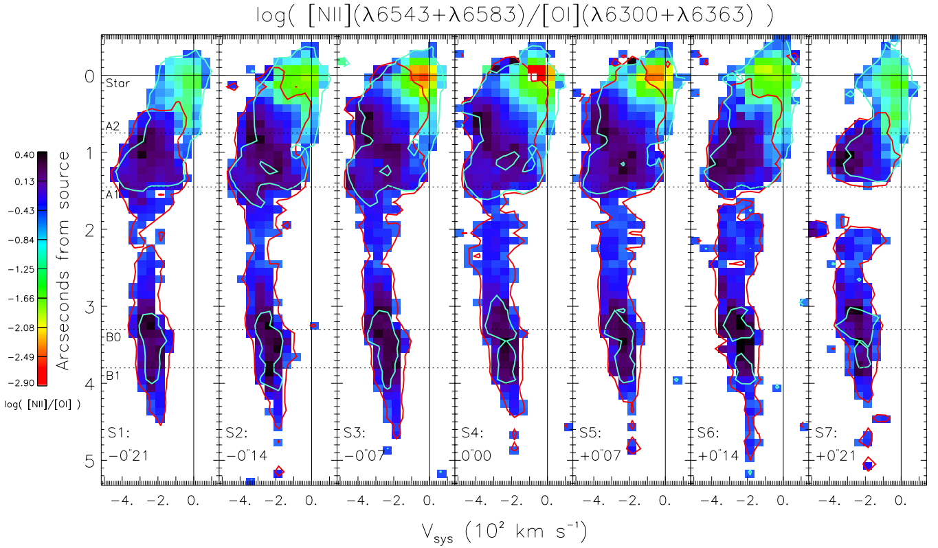
Fig. 5. Same as Fig. 4 for the logarithm of the [\text{NII}](\lambda 6583 + \lambda 6548) / [\text{OI}](\lambda 6300 + \lambda 6363) line ratio. The superposed cyan and red contours indicate the [\text{OI}]\lambda 6363 and the [\text{NII}]\lambda 6583 emission at 3\sigma ( [\text{OI}]\lambda 6300 = 3 [\text{OI}]\lambda 6363 and [\text{NII}]\lambda 6548 = 1/3 [\text{NII}]\lambda 6583 is assumed everywhere, see text).
