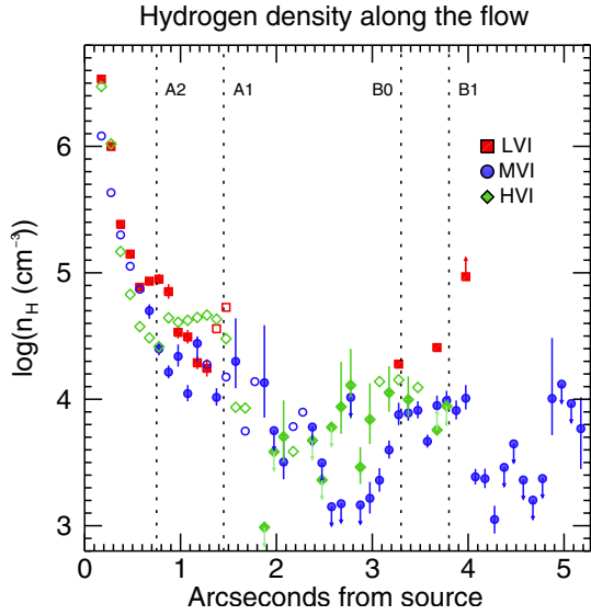
Fig. 13. Same as Fig. 11 for \log(n_{\text{H}}) .
