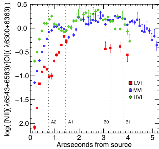
Fig. 17. Same as Fig. 16 for the logarithm of the [N\ II]/[O\ I] line ratio.
