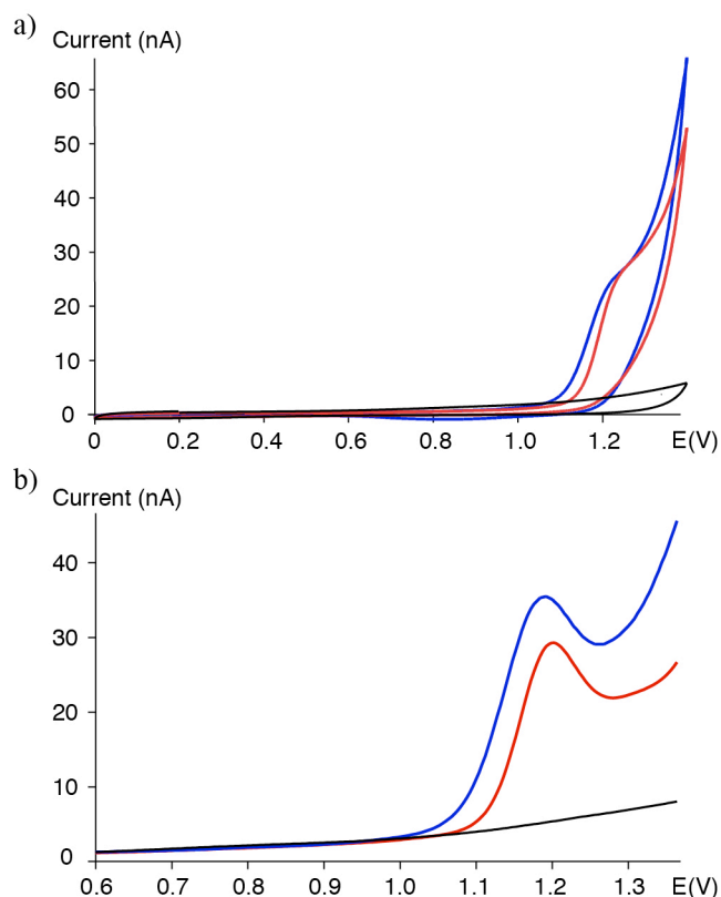
Fig. 3 a) Representative cyclic voltammograms (a) and differential pulse voltammograms (b) for complexes 1 (1.3 mM, blue) and 2 (1.1 mM, red) at pH 1.1 (0.1 M HNO 3 ), scan rate 30 mV s -1 , E(V) vs SCE (background current in black).
