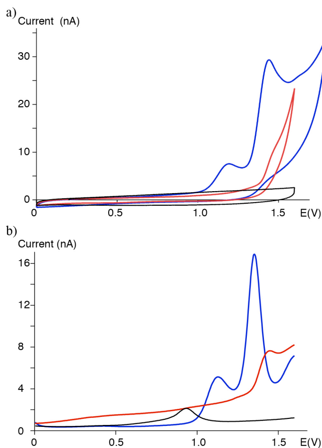
Fig. 6 Representative plots from cyclic voltammetry (a) and differential pulse voltammetry (b) for complexes 1 (1.4 mM, blue curve) and 2 (1.2 mM, red curve) in MeCN; 0.1 M \text{Bu}_4\text{N}(\text{PF}_6) as supporting electrolyte, 30 \text{ mVs}^{-1} scan rate, E(\text{V}) vs SCE.
