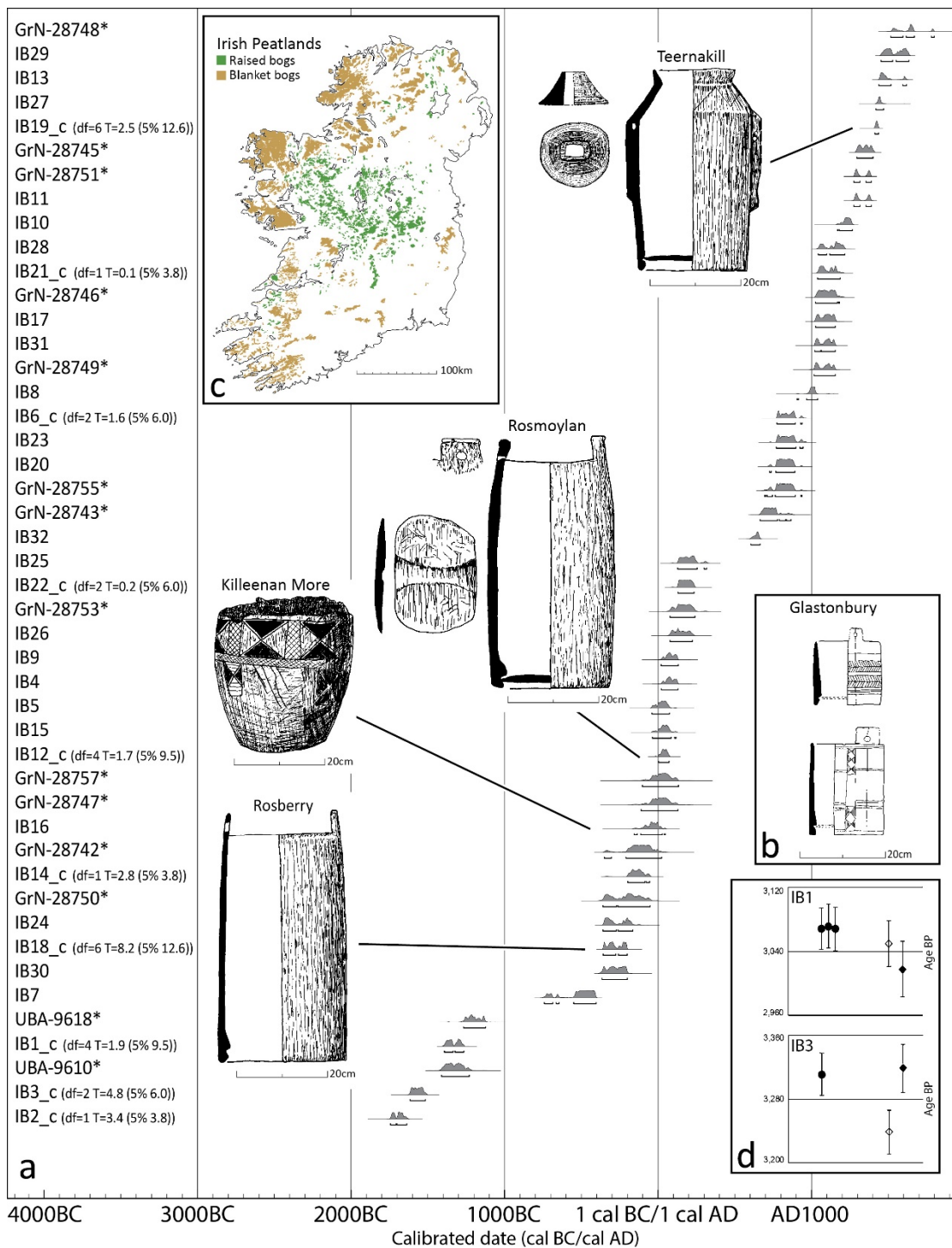
Figure 5: Dating of Irish bog butters. 5a: Radiocarbon date ranges for Irish bog butters, this study and additional specimens (marked with *; S2), with associated containers. Date ranges were calibrated using OxCal v4.3.2 and the IntCal13 atmospheric curve (56-57). 'C' denotes calculation of the weighted average of multiple measurements on the same bog butter, with the related chi-squared test results also displayed. T is the chi-squared value calculated and the value given in brackets is the level above which T should not rise in order to be acceptable. Degrees of freedom are given by df (number of dates minus one). All T results are below the respective values for rejection of the contemporaneity hypothesis at 2 \sigma confidence level. 5b: Iron Age wooden vessels from Glastonbury Lake Village, UK; 5c: Irish
