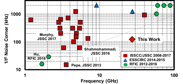
Fig. 1. Survey of 1/f 3 corner of the state-of-art RF and mmW oscillators.
