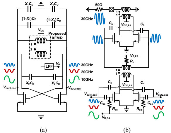
Fig. 3. Proposed 30GHz generation scheme: (a) 10GHz class-F 23 oscillator w/ proposed 1:2 transformer. (b) 30GHz two-stage PA.
