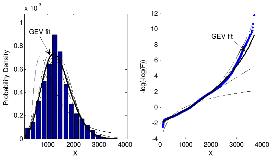
Fig. 2. Parent distribution of load effect 1 due to 2-truck events on a 20 m bridge (fits to alternative distributions shown dashed)
