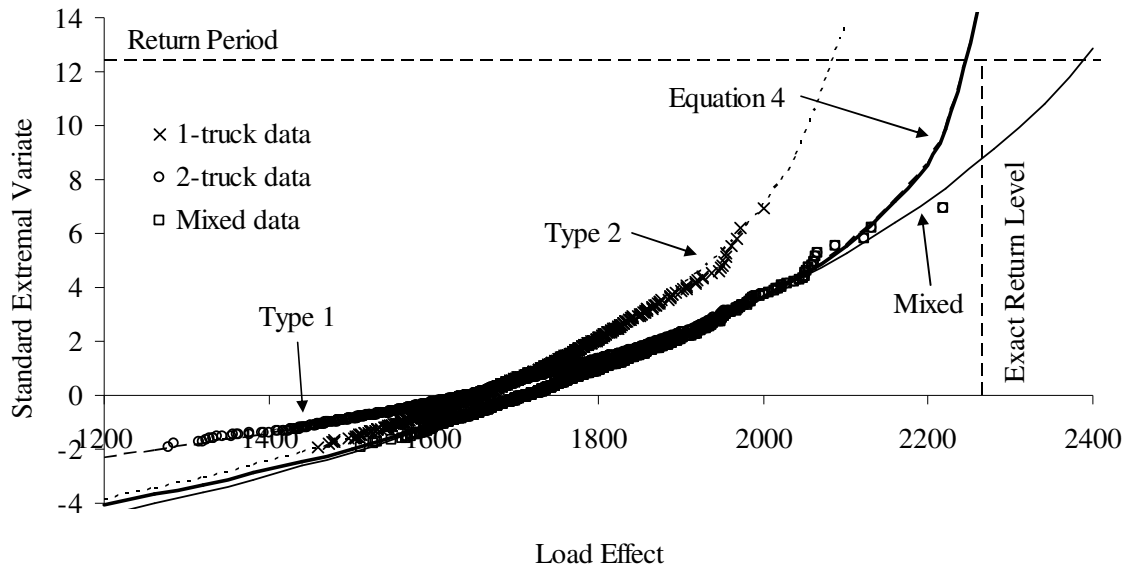
Fig. 5. Maximum-per-day simulated data from Example 2 on Gumbel probability paper
