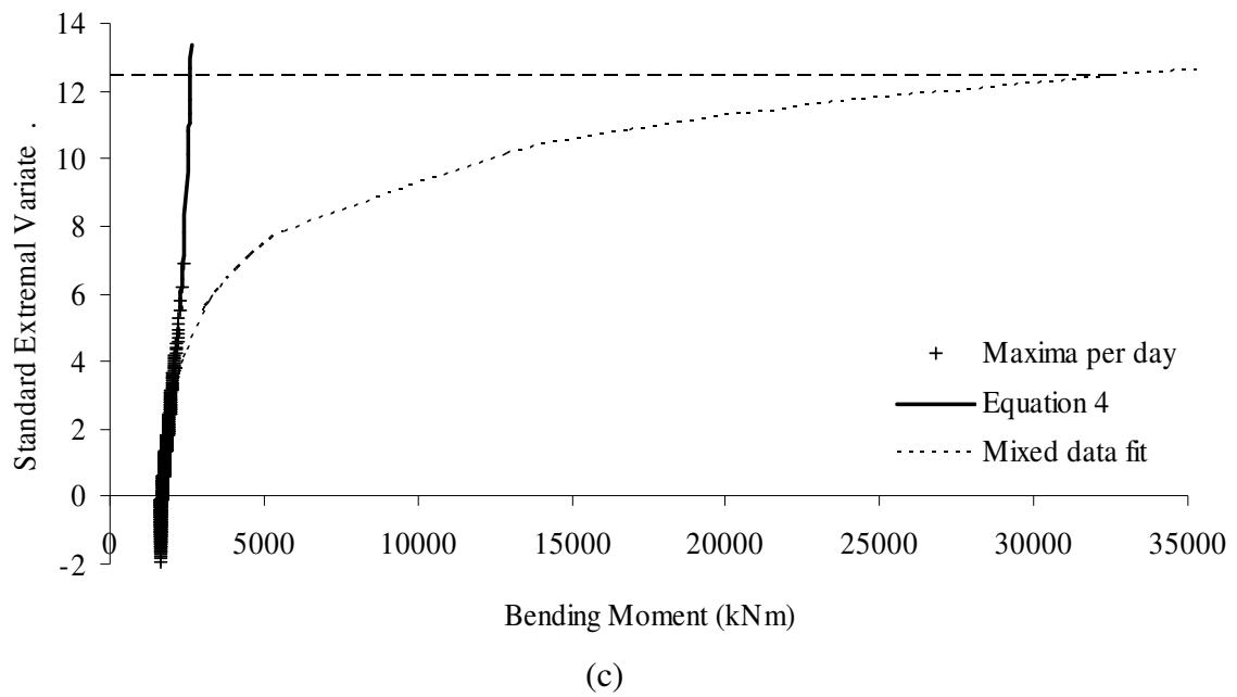
Fig. 4. Results for Load Effect 2 in a 40 m long bridge: (a) Daily maxima by event type; (b) Mixed daily maxima, (c) Mixed daily maxima extrapolation to characteristic values.
