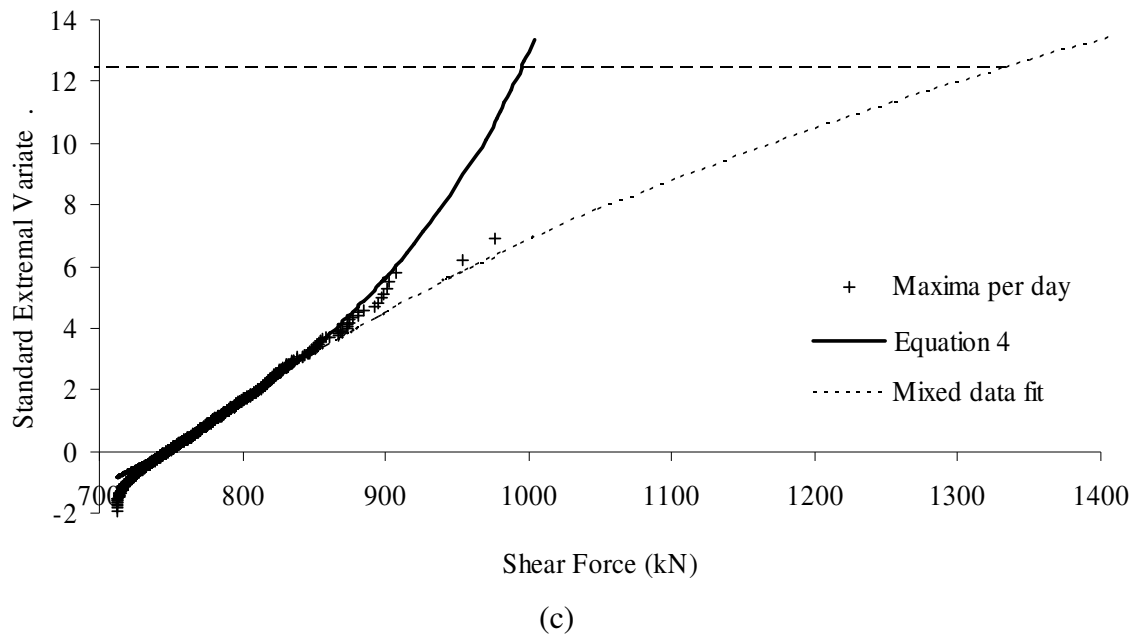
Fig. 3. Results for Load Effect 3 on 30 m long bridge: (a) Daily maxima by event type; (b) Mixed daily maxima; (c) Mixed daily maxima extrapolation to characteristic values.
