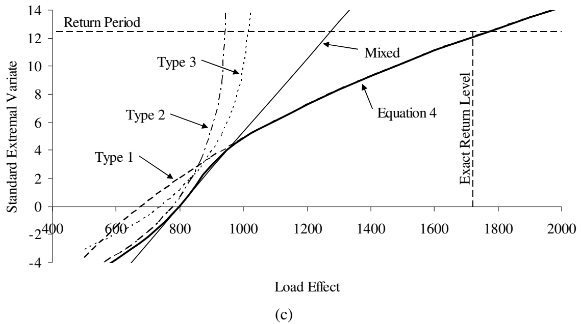
Fig. 1. Maximum-per-day simulated data from Example 1 on Gumbel probability paper: (a) detail of simulation period showing data; (b) detail of extreme values, and; (c) extrapolation to return level (omitting the data points for clarity).
