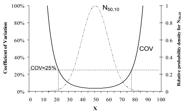
Fig. 2. Coefficient of Variation for a Normal distribution - N_{50,10}
