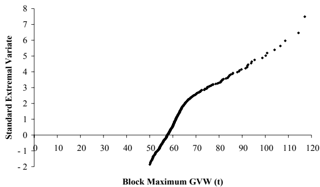
Fig. 3. Block maximum GVWs, both lanes combined, Branisko, on Gumbel probability paper
