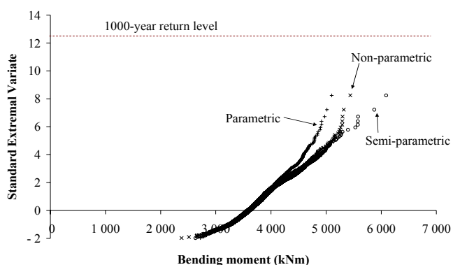
Fig. 4. Daily maximum mid-span bending moments, simply supported 35 m span, single truck load, fast lane, Woerden.
