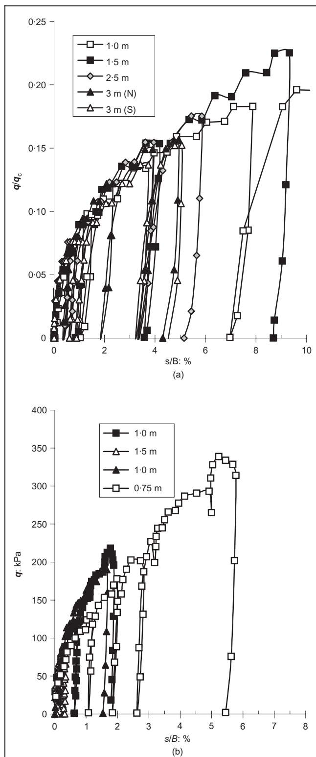
Figure 6. Pressure–settlement curves from footings tests in Table 1: (a) Texas, Site A; (b) Shenton-Park, Site C
