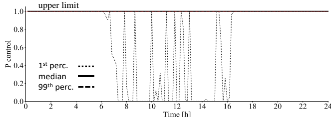
Fig. 8. 1 st , 50 th and 99 th percentiles for all PVs P_{control_{pv}}
