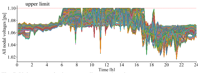
Fig. 7. Voltage magnitudes across all network nodes
