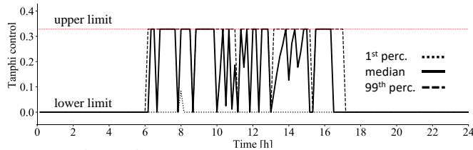
Fig. 9. 1 st , 50 th and 99 th percentiles for all PVs Tan\phi_{control_{pv}}
