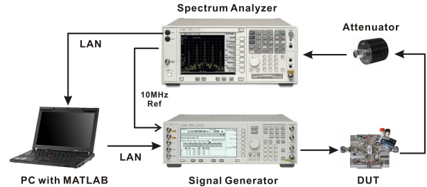
Figure 6. Example of commercial instruments-based DPD platform.
