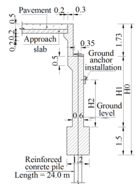
d. Cross section of proposed abutments
