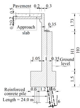
c. Cross section of traditional abutments (*)
